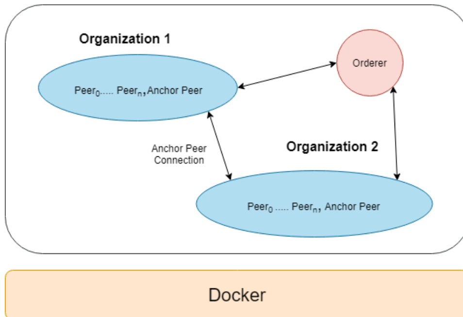
Figure 4. Entities in HLF represented as Docker containers
