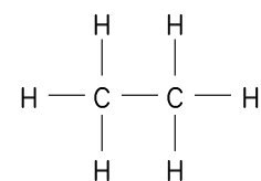
ETHANE, C_2H_6
