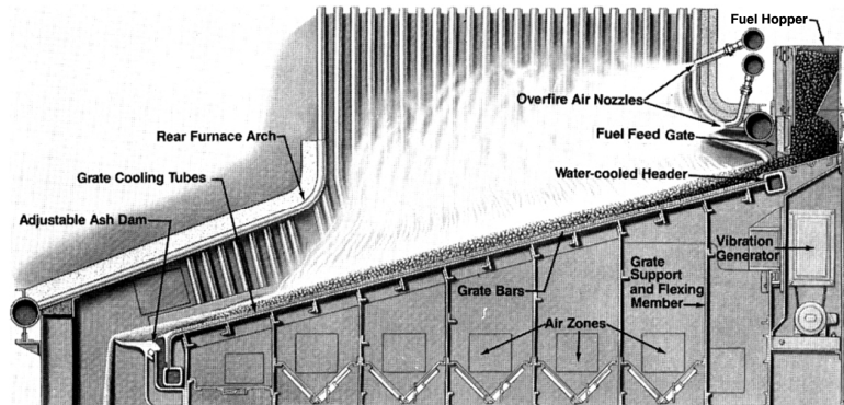
Figure 5-3. Cross Section of Overfeed, Water-Cooled, Vibrating-Grate, Mass-Feed Stoker
