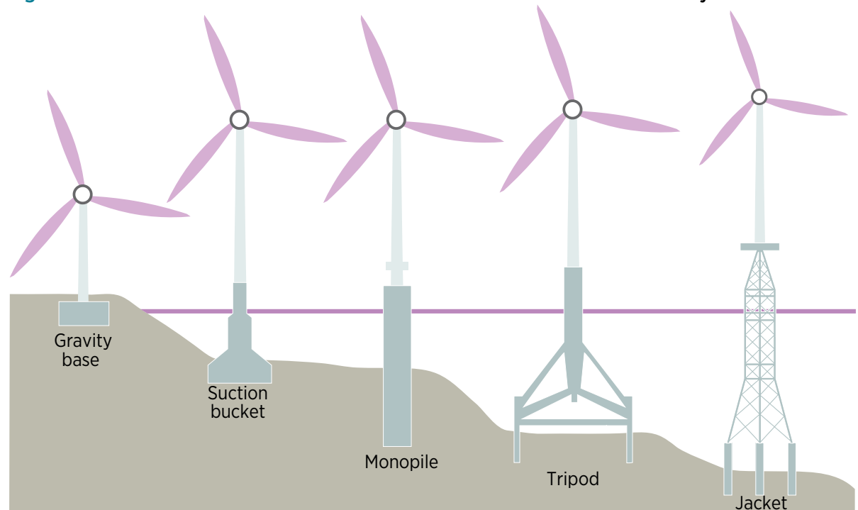
Figure A.1 ■ Fixed-bottom foundations used in the offshore wind industry
