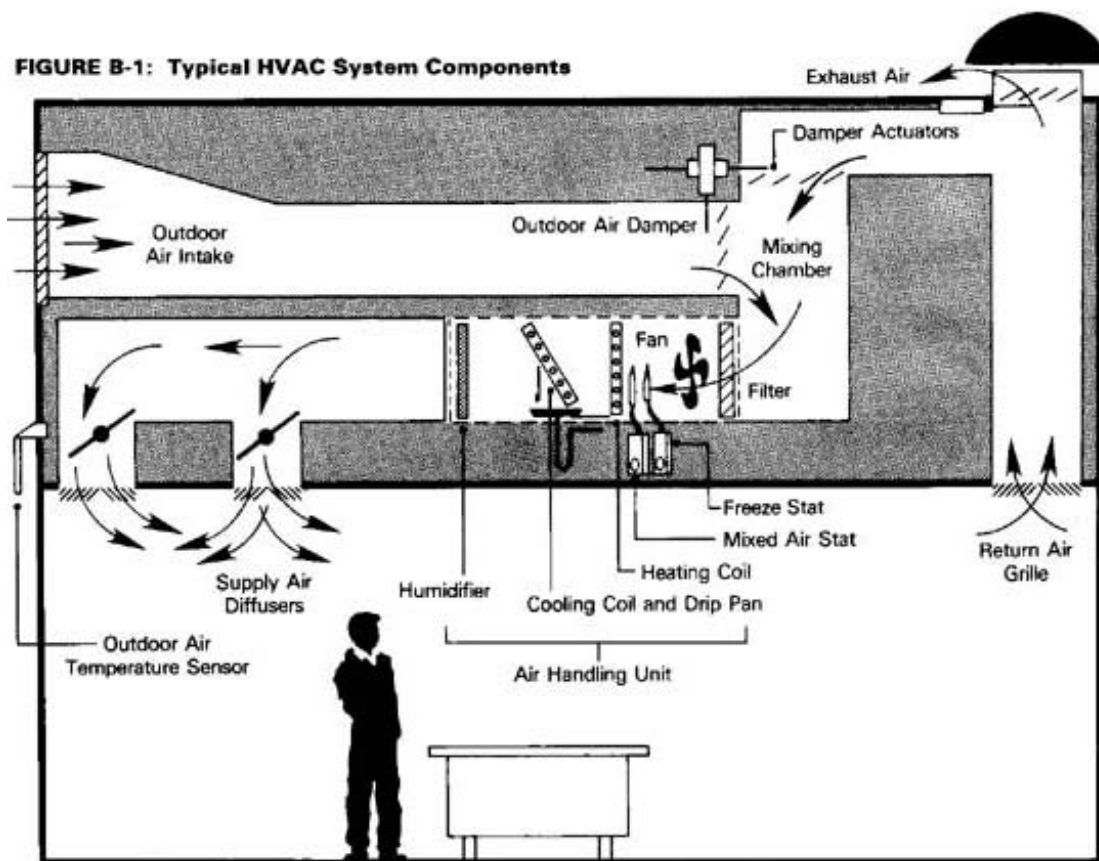
FIGURE B-1: Typical HVAC System Components
