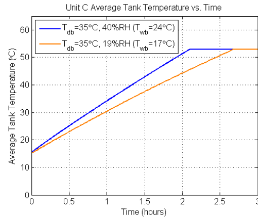
Figure 24. Effect of humidity on recovery time for Unit C
