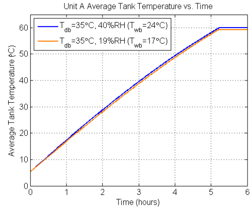
Figure 36. Effect of humidity on recovery time for Unit E
