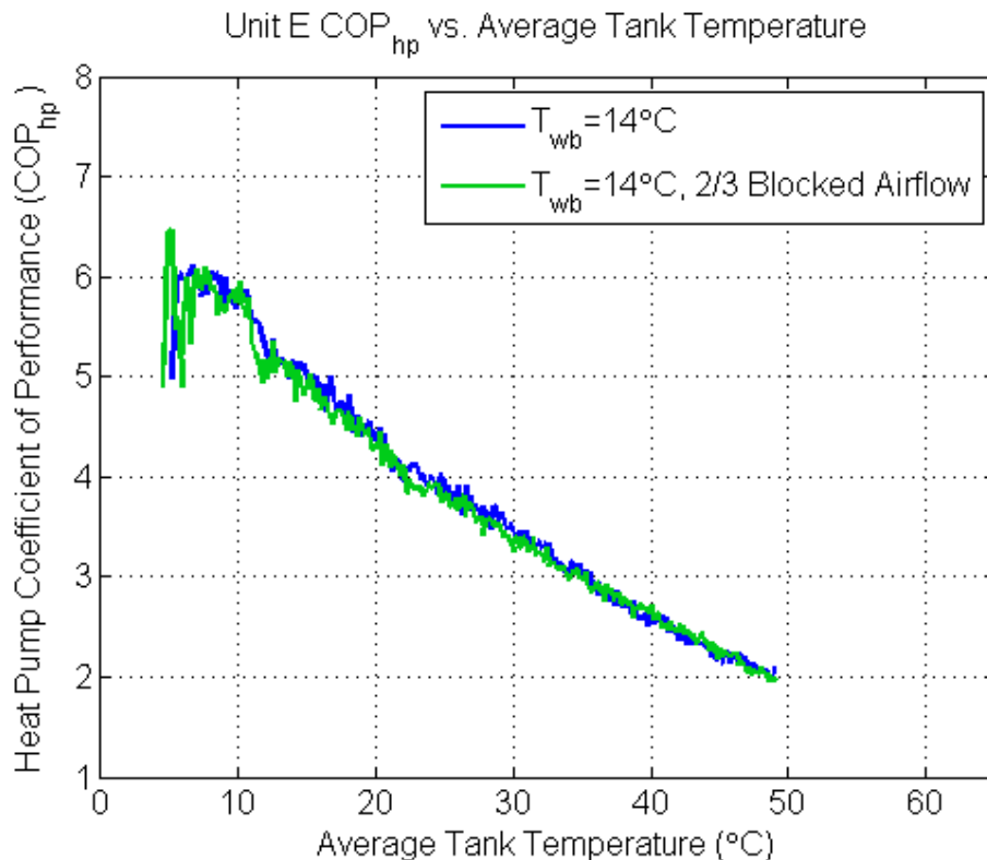
Figure 37. COP_{hp} traces Unit E with reduced airflow
