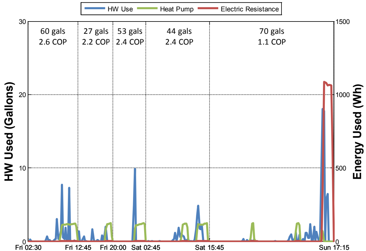
Figure 23. Example of five heating events as defined in this study
