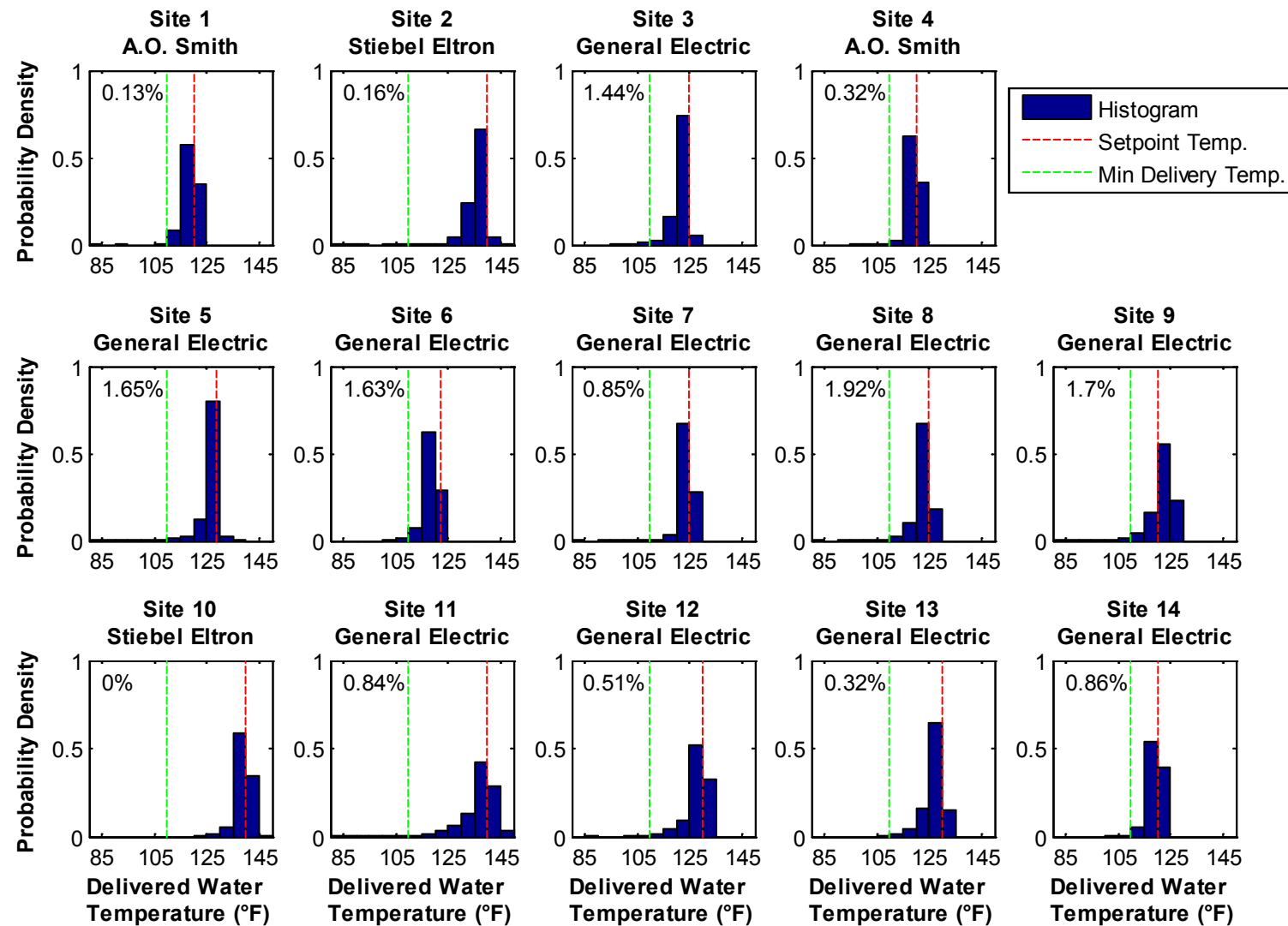
Figure 14. Normalized histograms of delivered water temperature. Red line indicates set point temperature. Green line indicates minimum delivery temperature (110°F). The percentage of occurrences with water temperatures lower than 110°F is shown.
