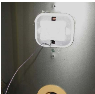
Figure 3. The insulation is replaced and the TC wire is directed through a hole in the insulation.
