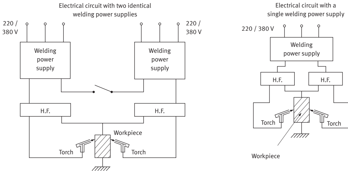
Fig. 3.1.4 - Principle of simultaneous two-operator TIG welding – Two operators weld in one pool on both sides at the same time
