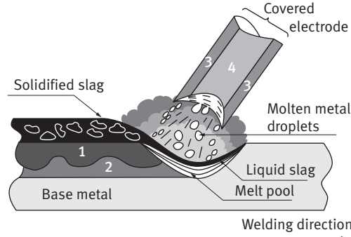
Fig. 3.1.15 - Principle of the (S.M.A.W.: Shielded Metal Arc Welding) process 1 – Solidified deposit metal 2 – Mixing zone 3 – Flux covering 4 – Electrode core
