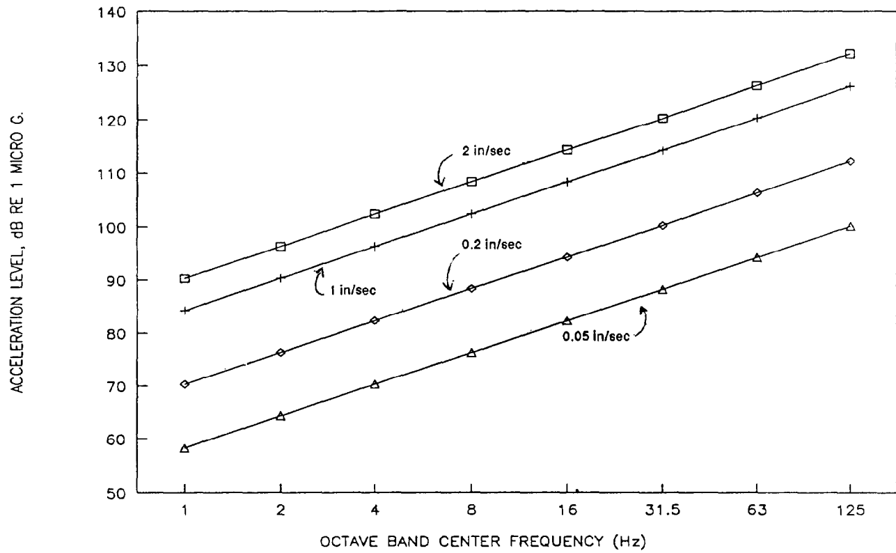
Figure 2-4. Vibration Criteria for Damage Risk to Buildings.
