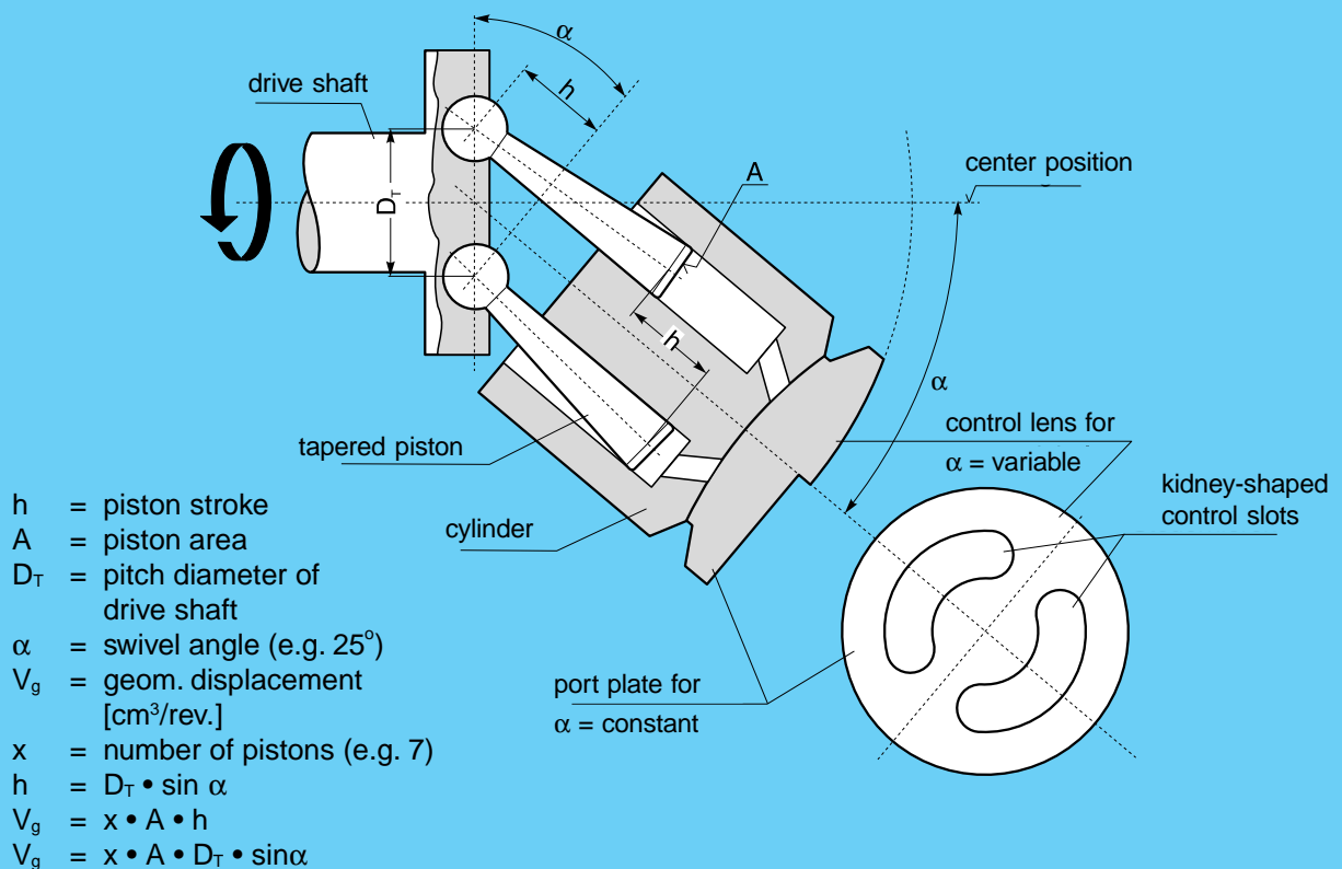
Schematic Diagram of a Bent-Axis Unit with fixed or variable swivel angle \alpha
