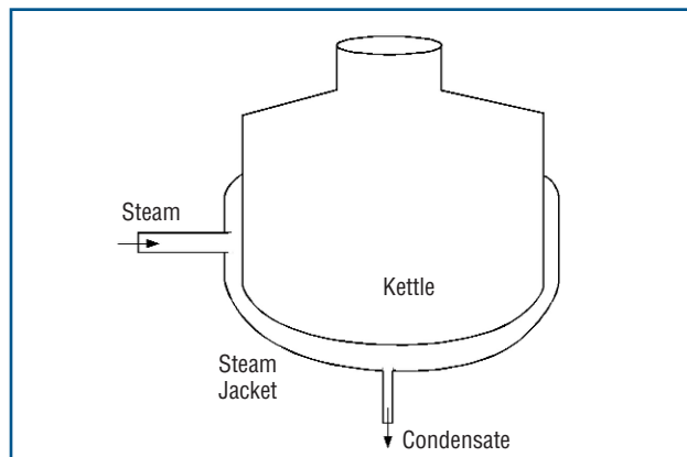
Figure 11. Configuration of a Jacketed Kettle Heat Exchanger
