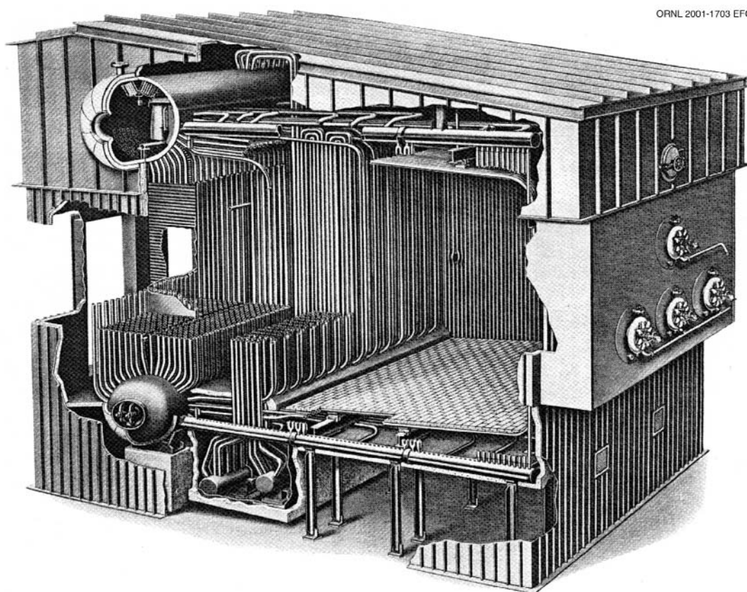
Figure 3. Watertube Boiler 6
