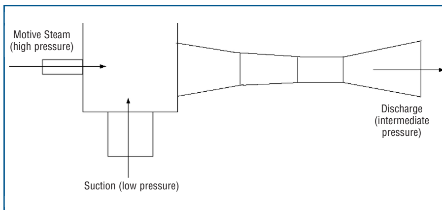
Figure 12. Thermocompressor Operation
