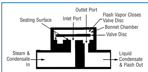
Figure 8. Thermodynamic Disc Steam Trap
