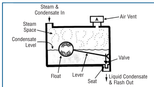
Figure 7. Float and Thermostatic Steam Trap
