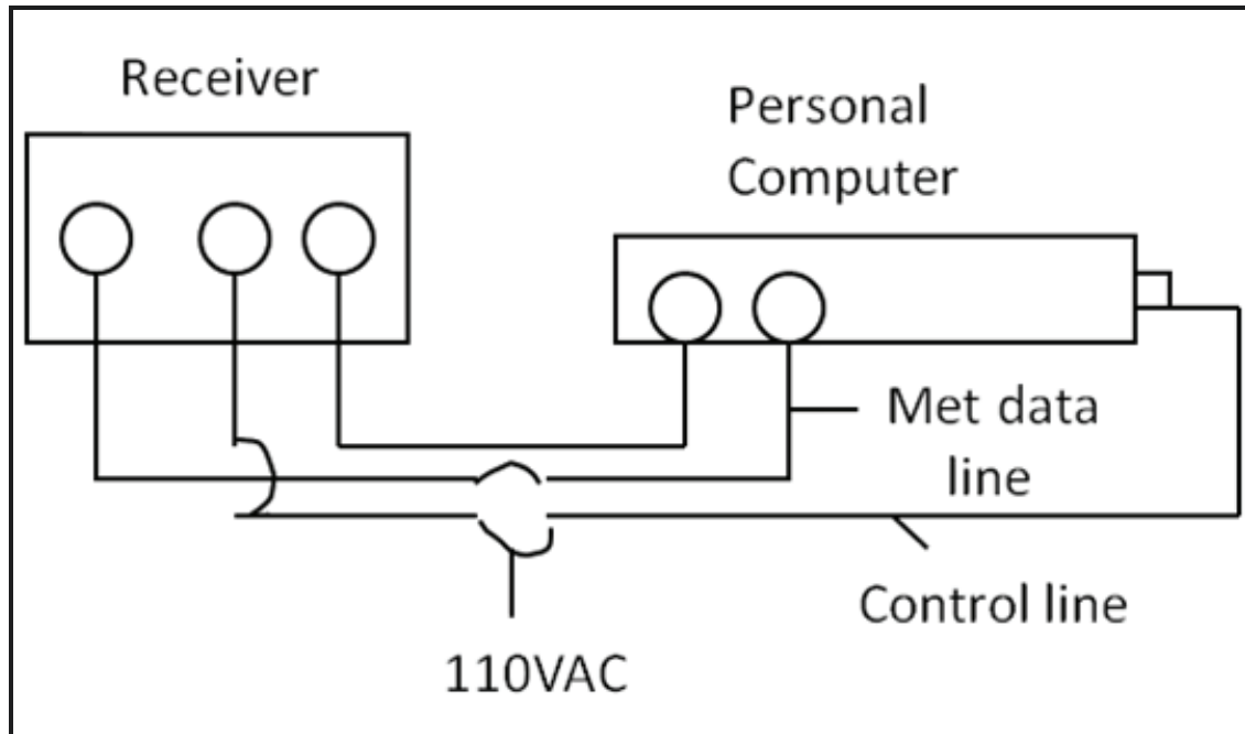
Figure 2-7. Connection diagram for the tethersonde electronics. Beware: 9-pin control line, marked with red tape, has a short special cable section on the PC end with a very fragile connector that goes into the PC mother board through the side of the PC.
