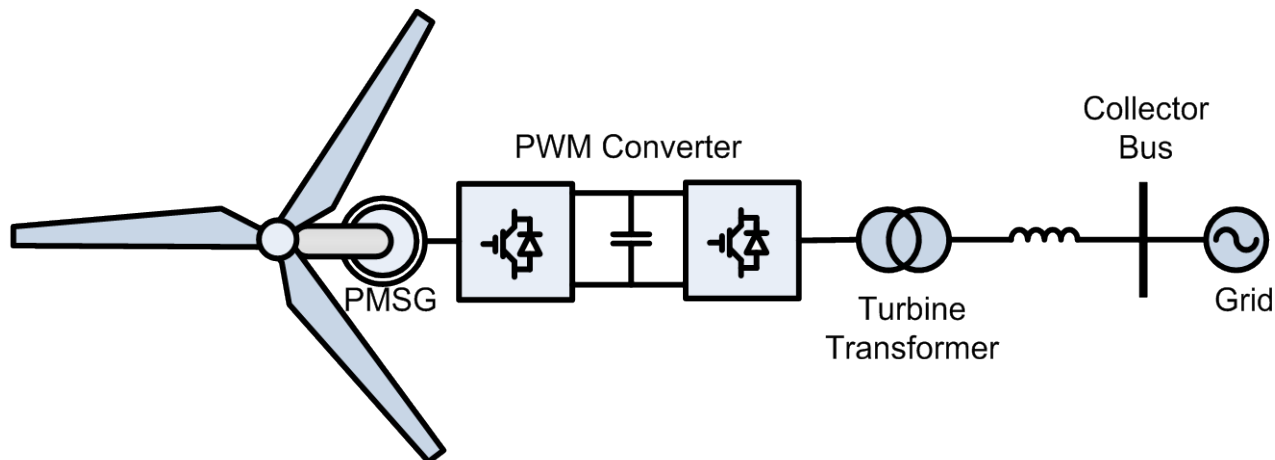
Figure 47. Type 4 wind turbine connection diagram
