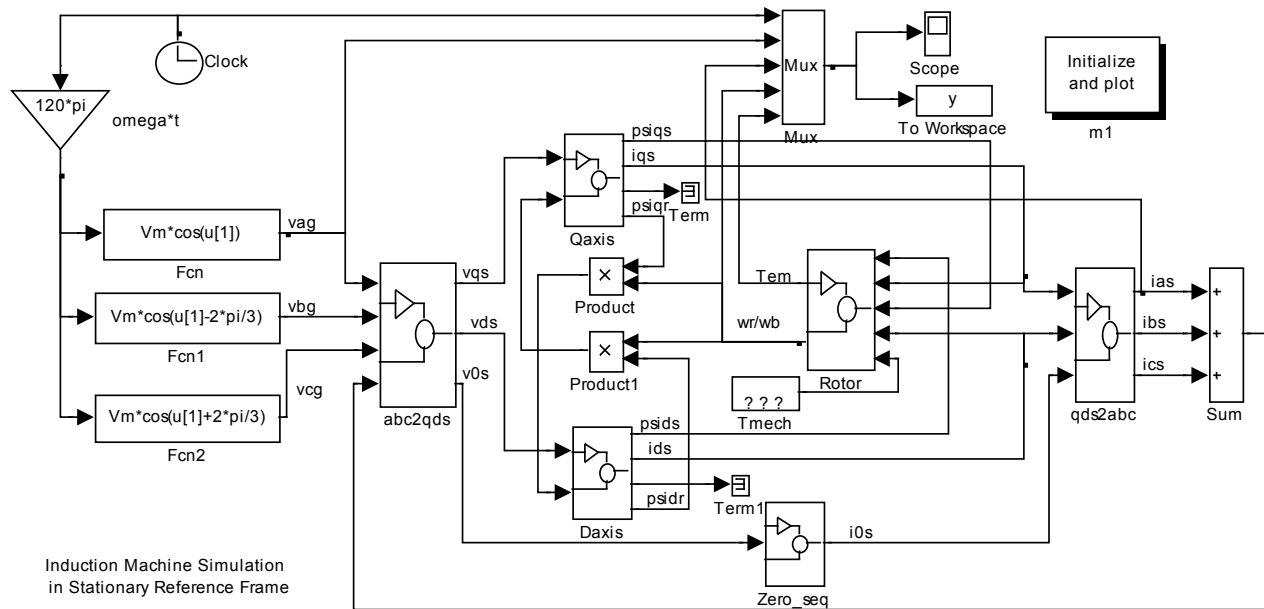
Figure 19. Induction machine model S1.mdl
