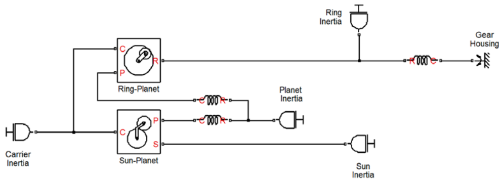
Figure A.15. One meshing set of a planetary gear set
