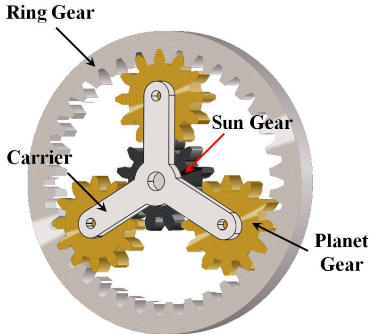
Figure 62. Planetary gear set with three planet gears
