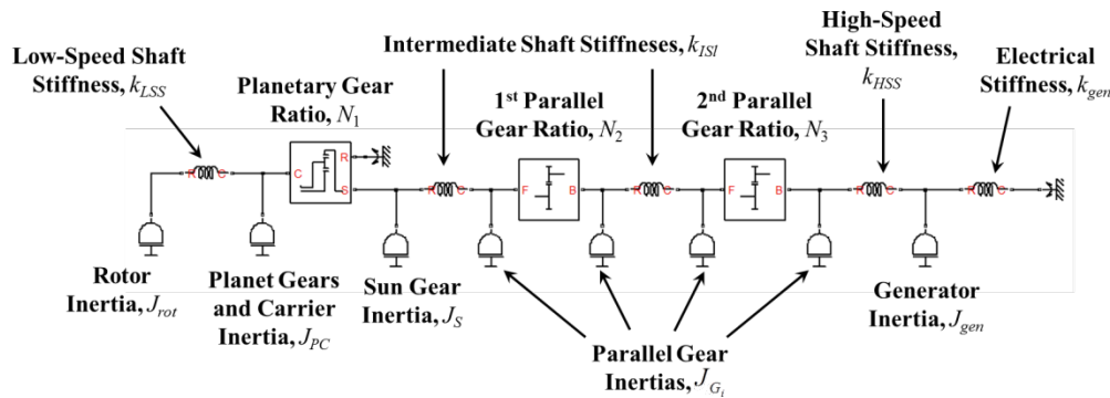
Figure A.3. SimDriveline model of a wind turbine drivetrain
