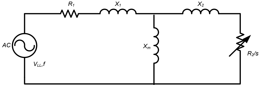
Figure 15. Induction machine single-phase equivalent circuit
