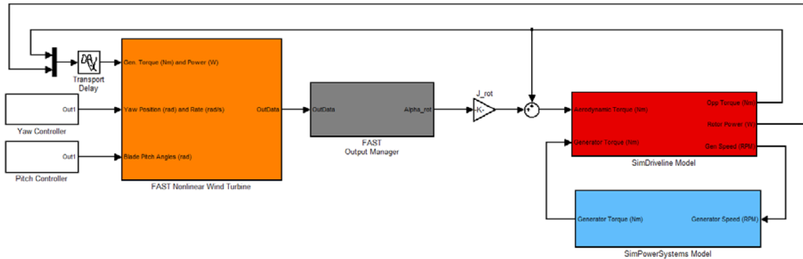
Figure A.23. Implementation of an integrated wind turbine drivetrain model
