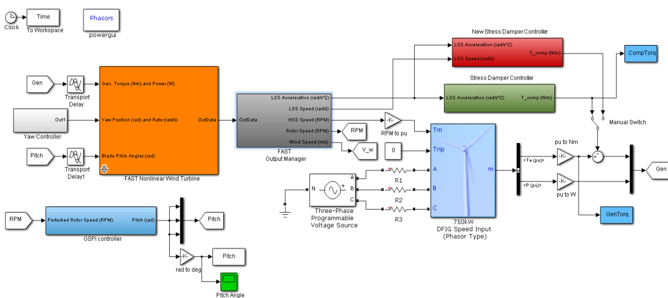
Figure 46. Type 3 wind turbine model using SimPowerSystems
