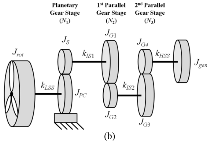
Figure A.1. (a) Modular wind turbine drivetrain and (b) multistage representation of the drivetrain
