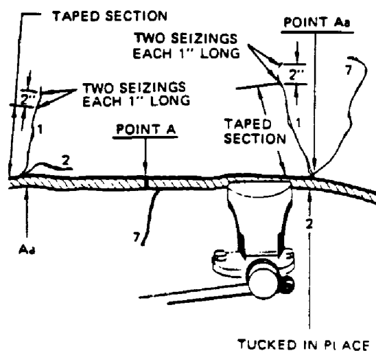
Figure 613-1-39. Vice Position
