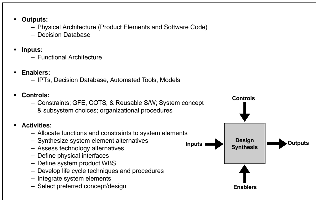
Figure 6-1. Design Synthesis
