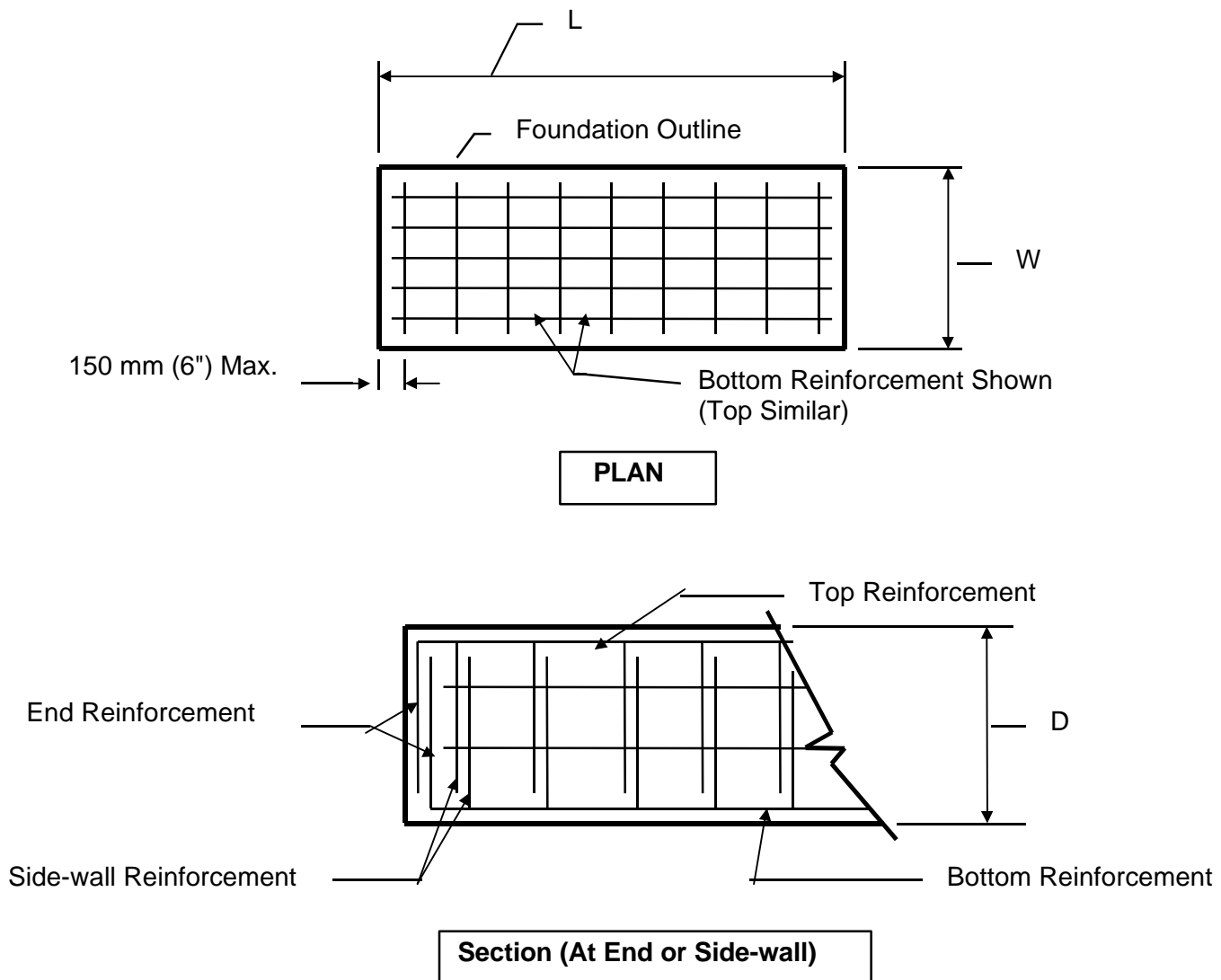
Figure 3-1. Machinery Foundation Reinforcing.
