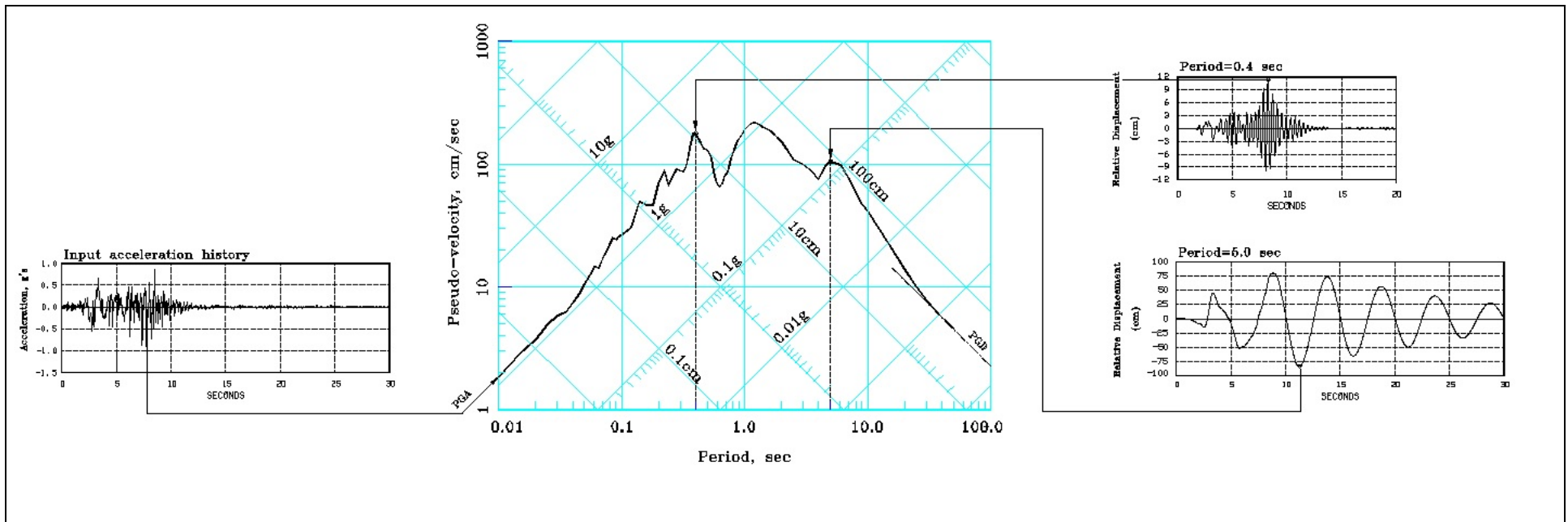
Figure 7. Constructing Site-Specific Ground Motion Response Spectrum
