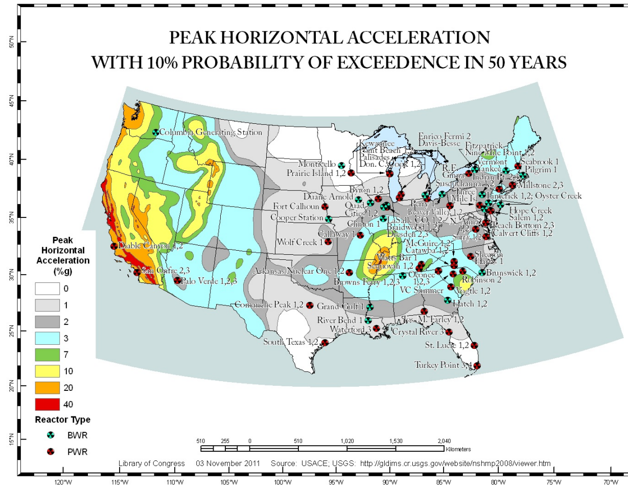
Figure 10. Operating Nuclear Power Plants vs. Seismic Hazard
