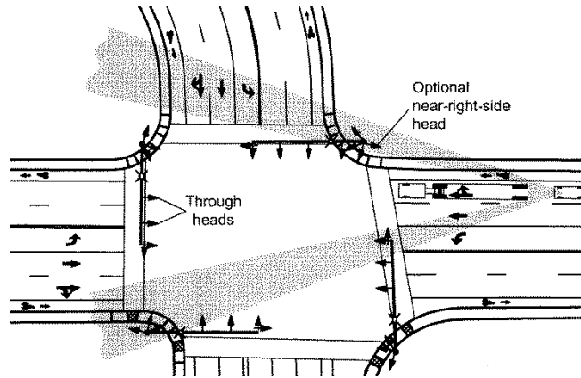
(a) Optional Head #1: Near-side head for through vehicles.
