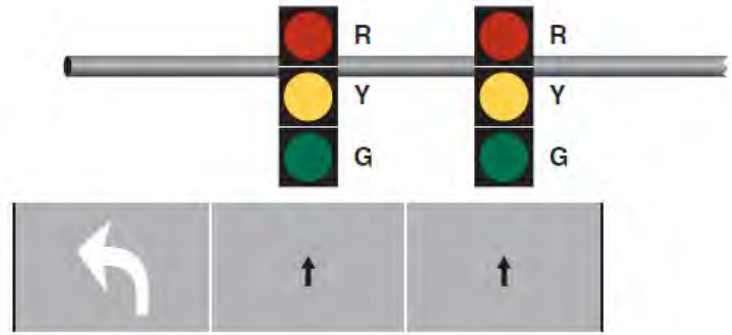
(a) Permissive left-turn phasing using three-section signal heads over the through lanes only.
