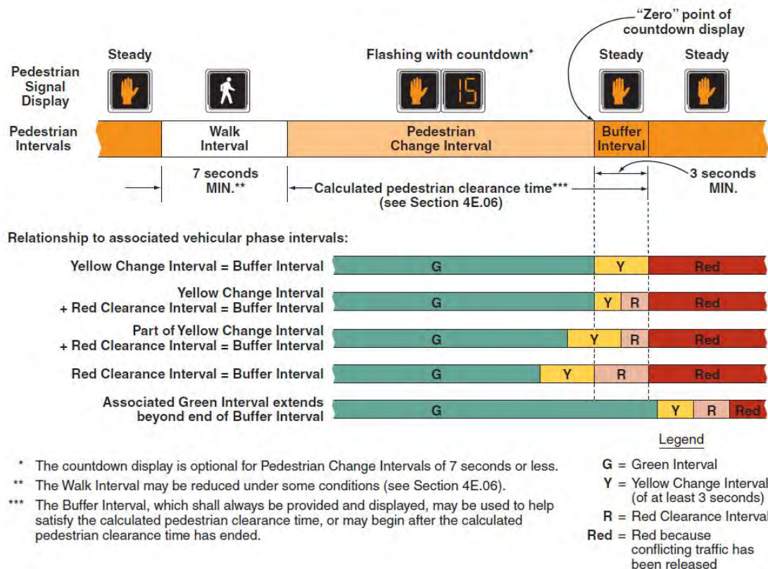
Exhibit 5-19. Pedestrian intervals. Source: 2009 MUTCD
