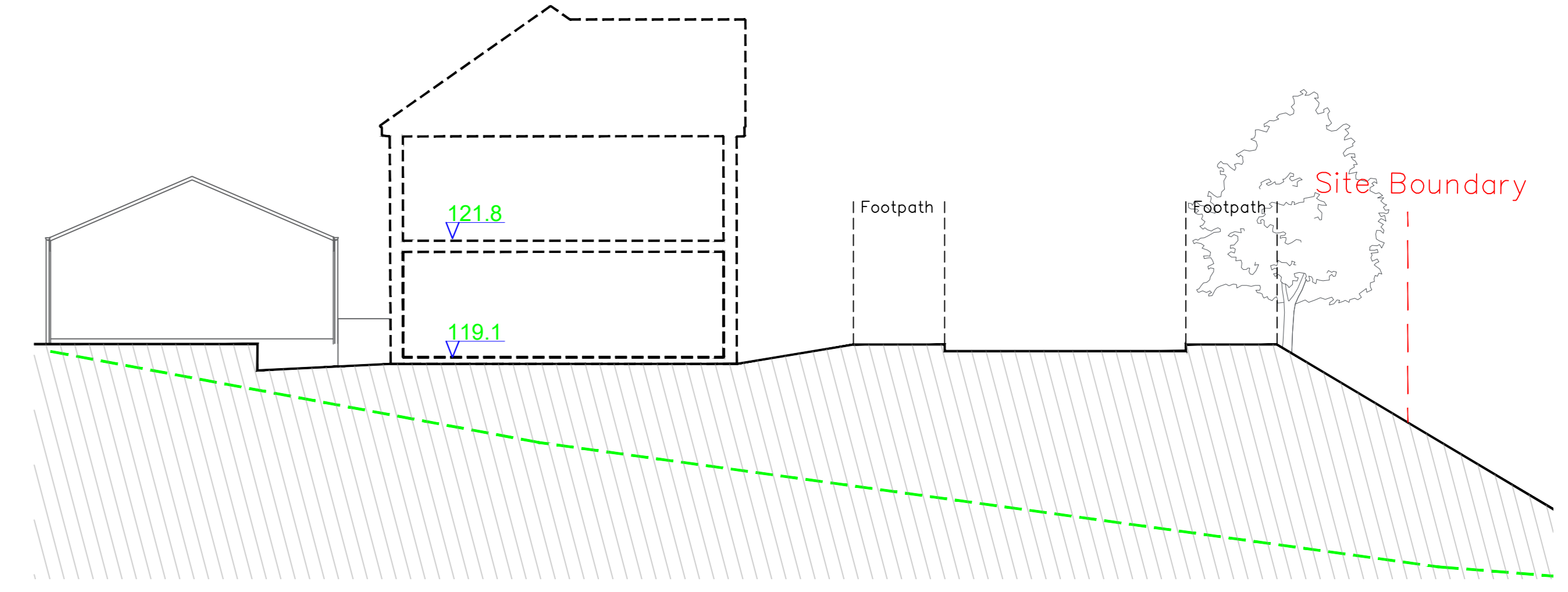
Site Section C-C
