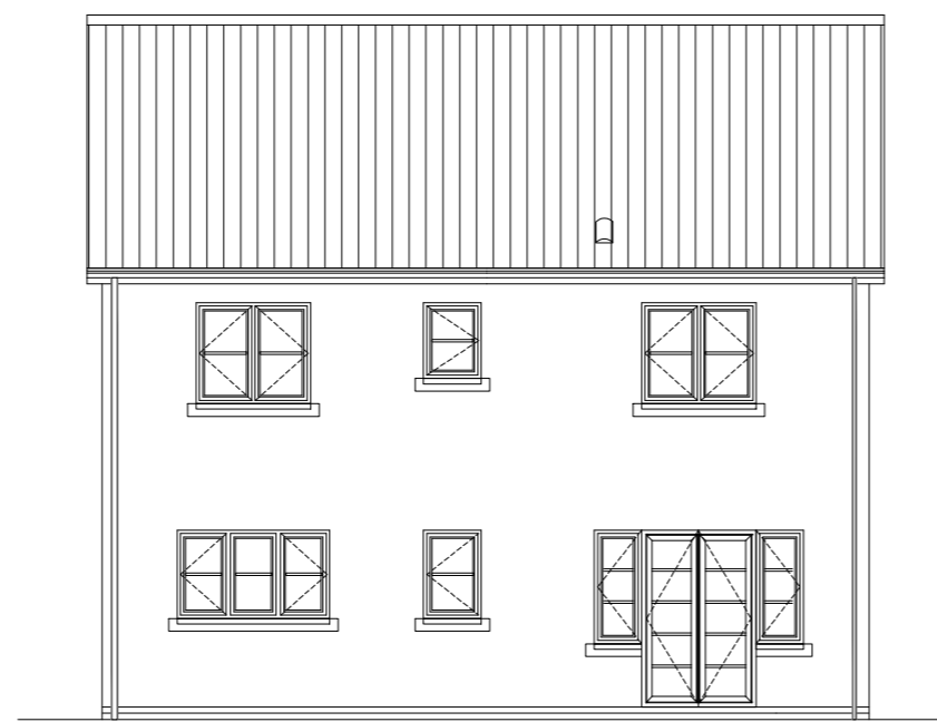
REAR ELEVATION
