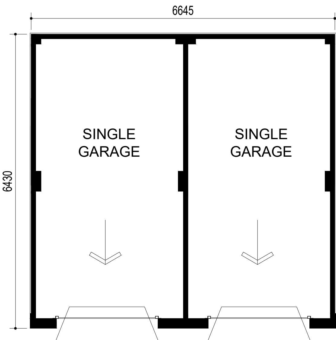
FLOOR PLAN
