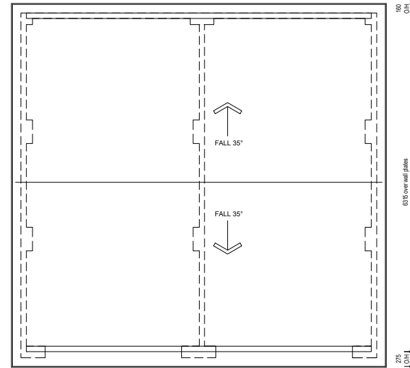
Roof Plan
