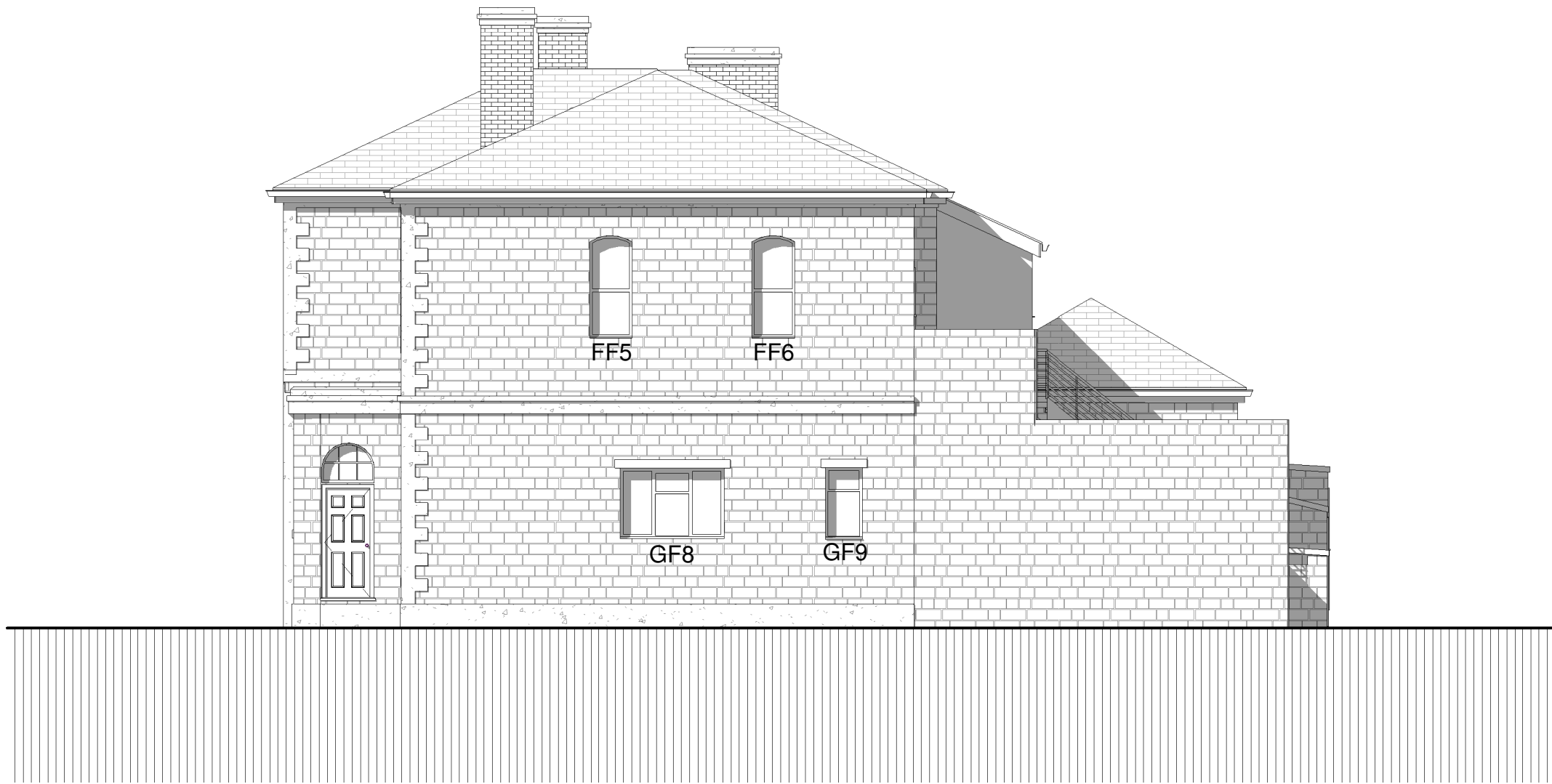
Existing West Elevaton 1 : 100
