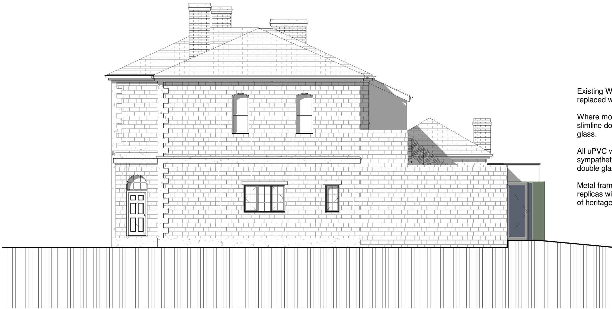
Proposed West Elevation 1 : 100
