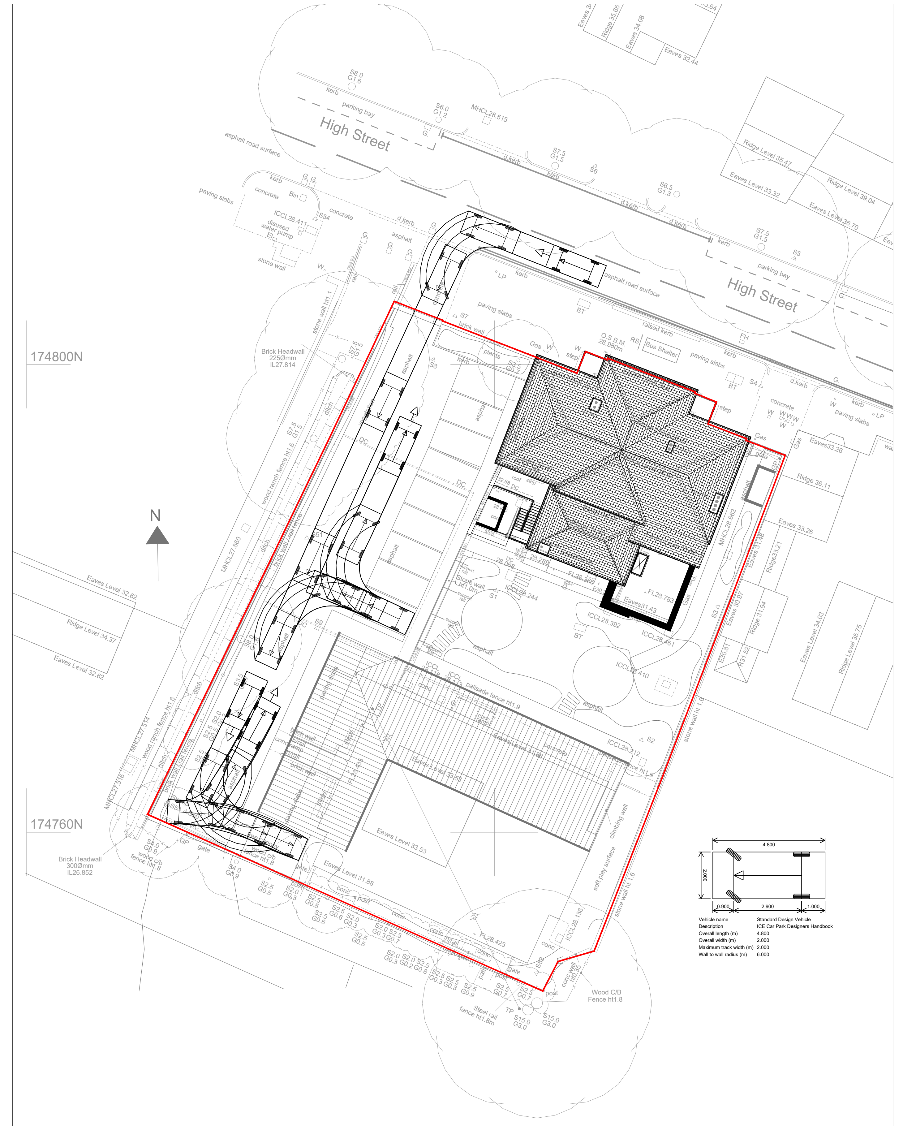
ICE Standard Design Vehicle Tracking Scale 1:200
