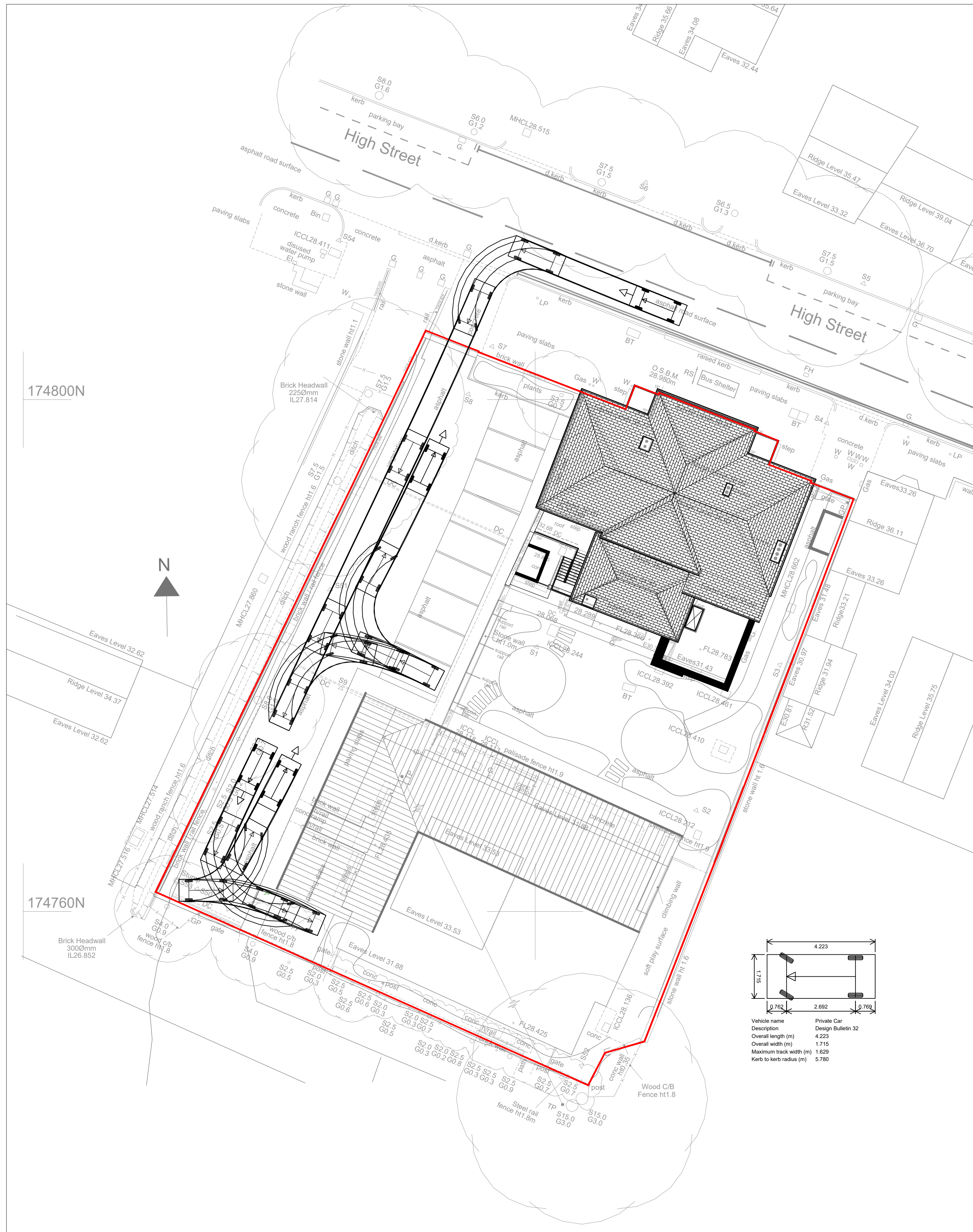
DB32 Private Car Tracking Scale 1:200
