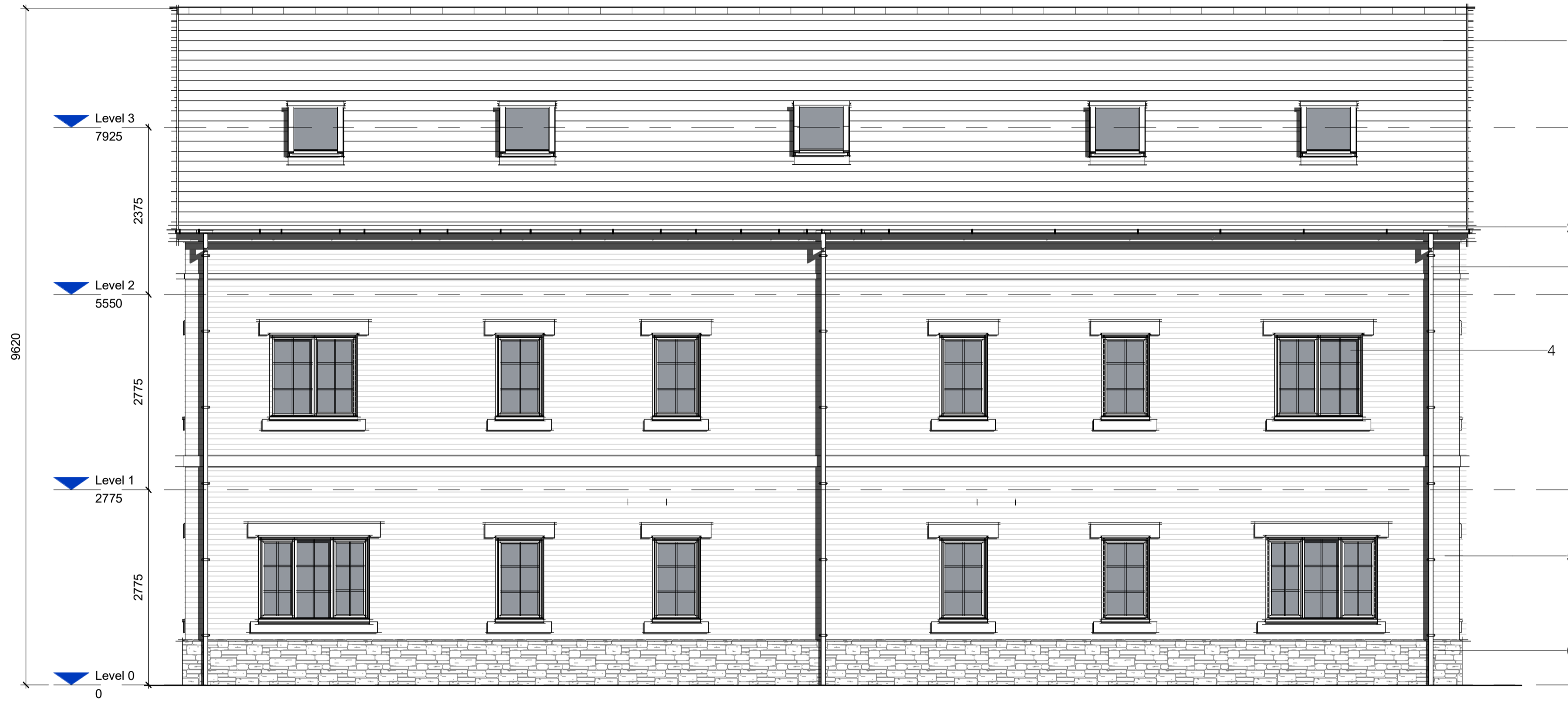
Rear elevation (Block 1 & 2)
