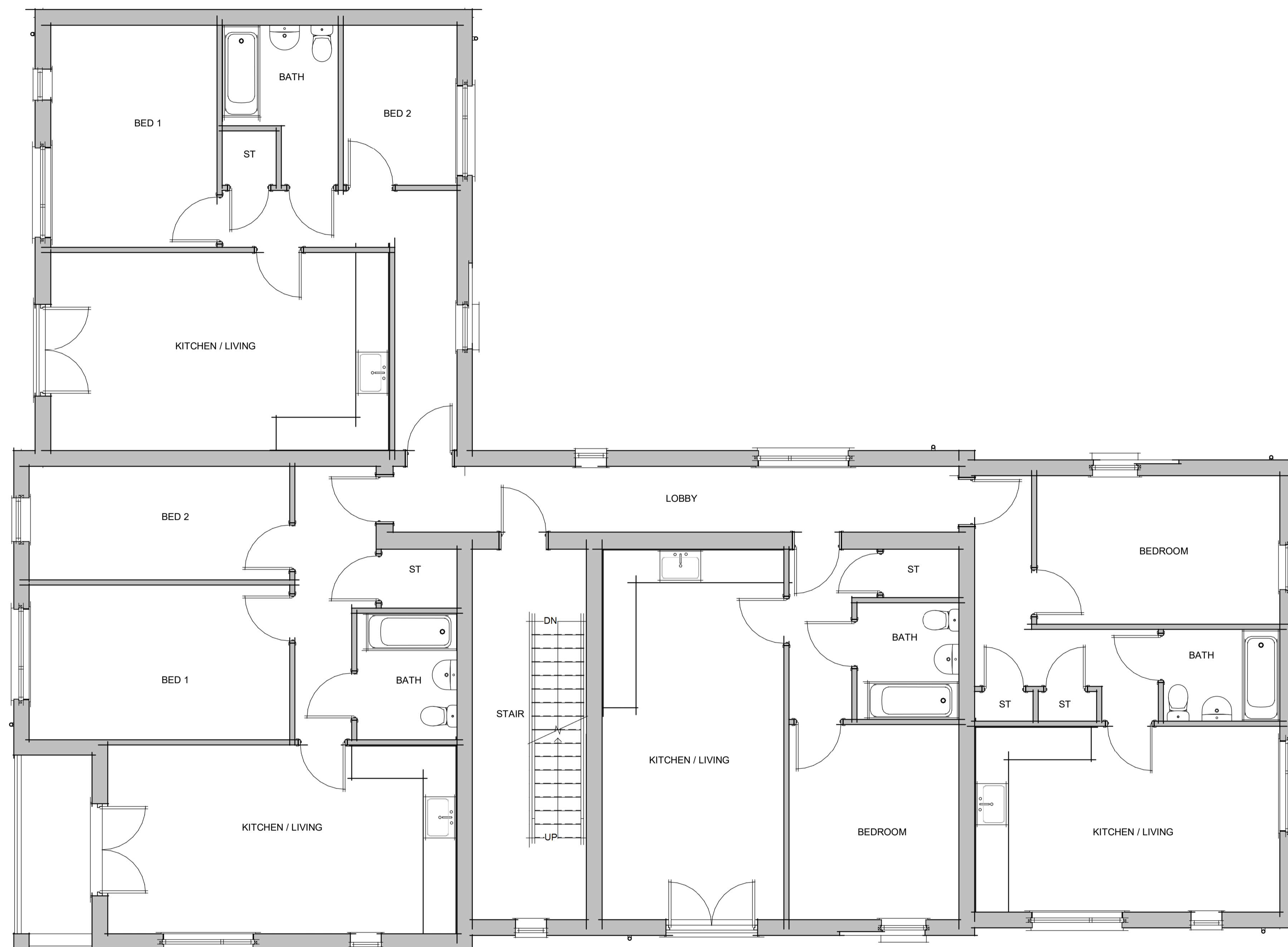
01 First floor plan 1 : 50
