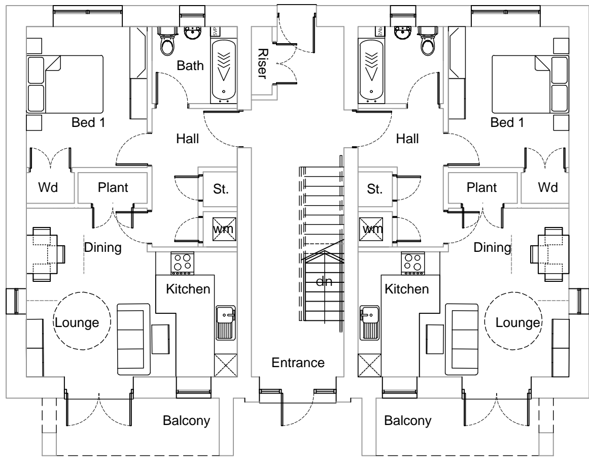
BUILDING TYPE B: GROUND FLOOR PLAN
