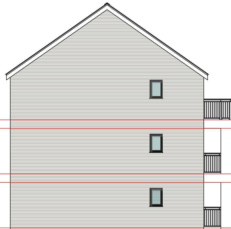
BUILDING TYPE B: SIDE ELEVATION
