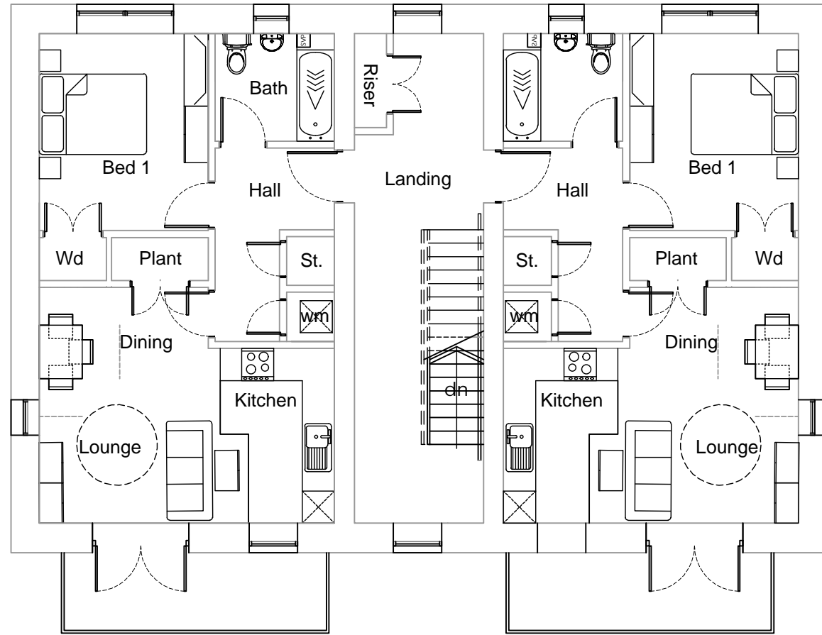
BUILDING TYPE B: SECOND FLOOR PLAN
