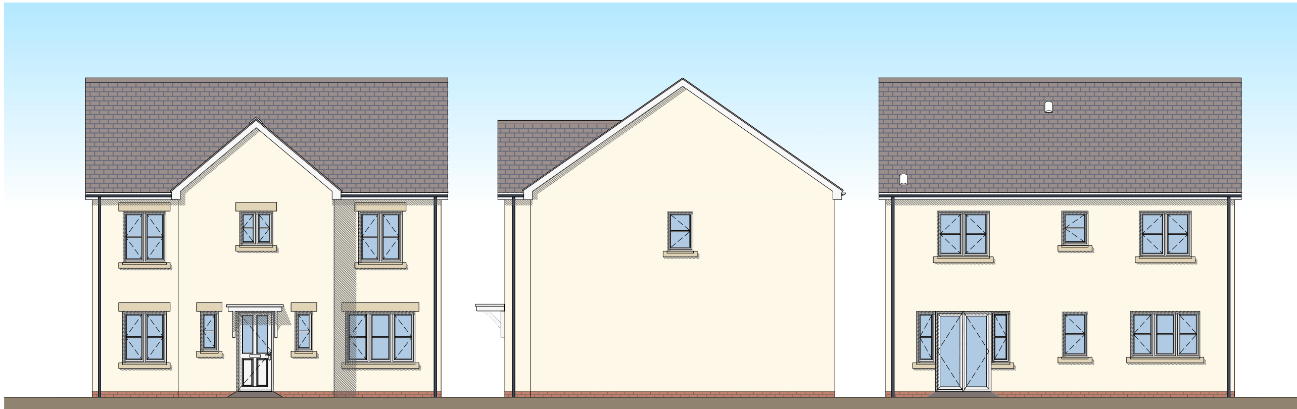
Front Elevation
