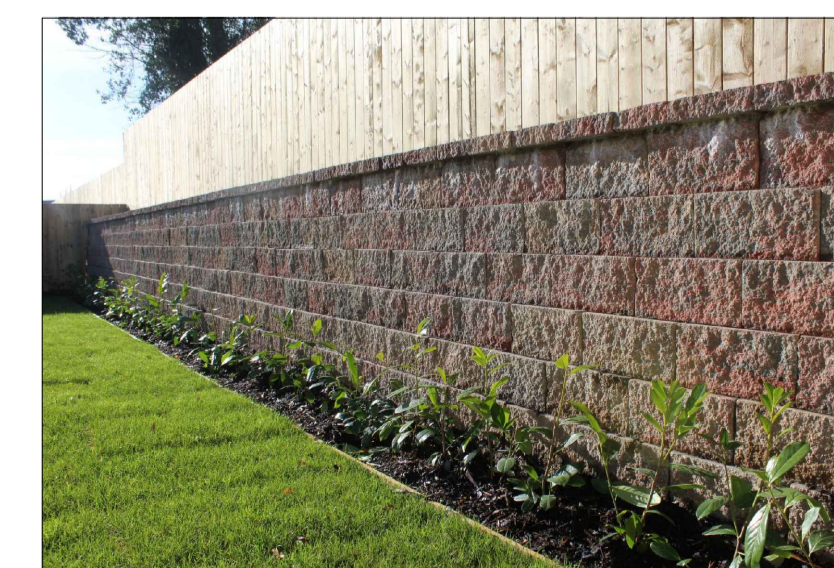
Retaining Wall to rear Tobermore Secura Colour - Heather
