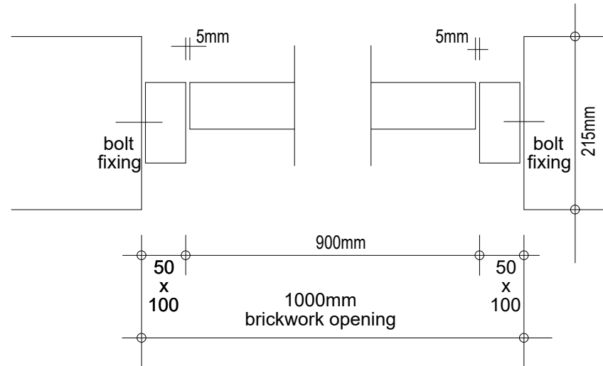
PLAN DETAIL 02
