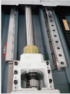
3 linear guideways for X and W axis
