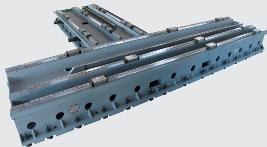
3 linear guideways for X and W axis
