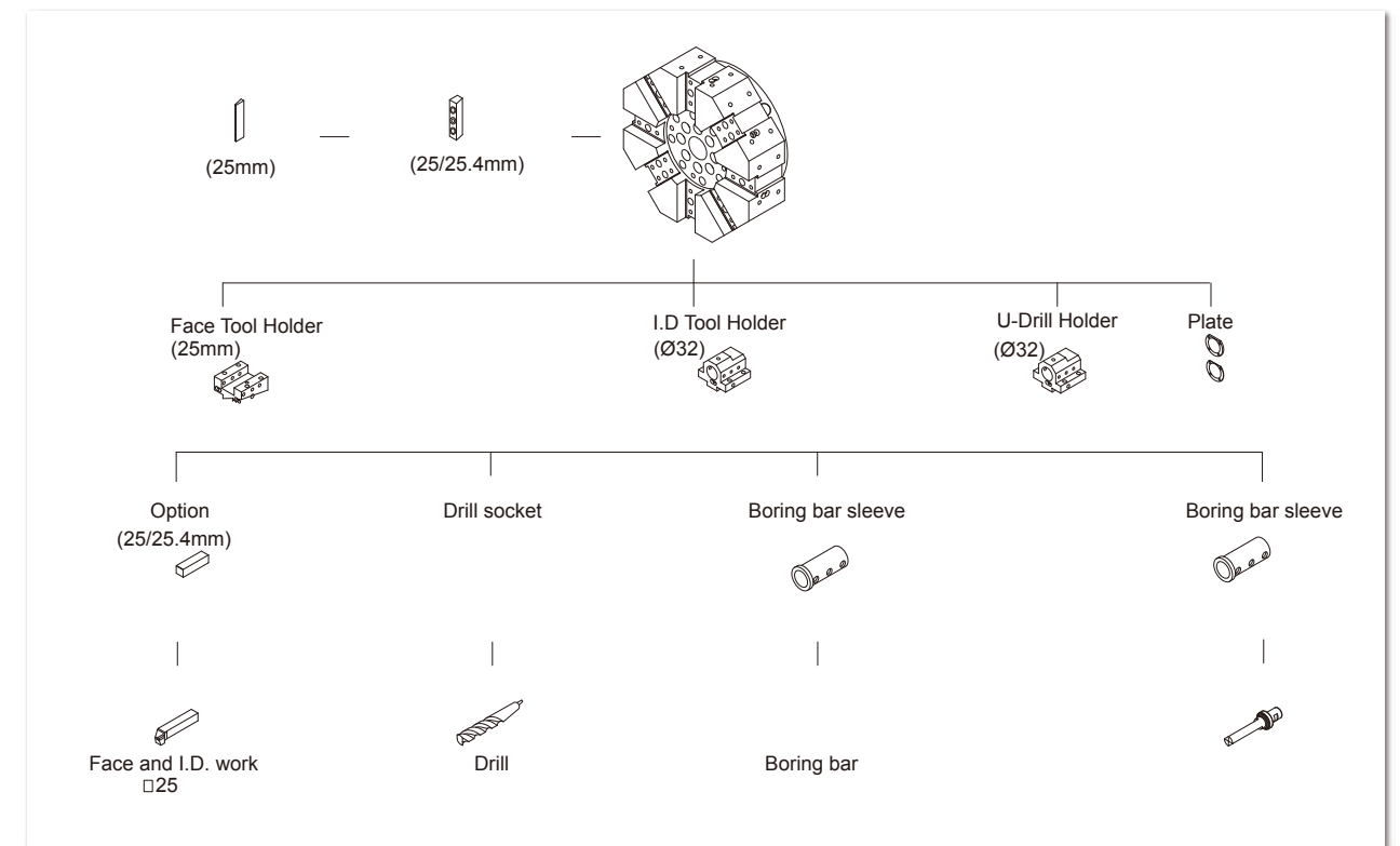
BNC-1800 with TB-160 8-station turret VDI40 disc
