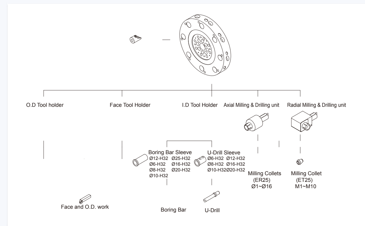
BNC-1600 with TB-120 8-station turret VDI30 disc
