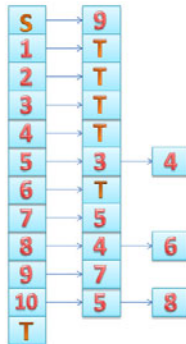
Fig. 5. Output of all maximum non-crossing subsets
