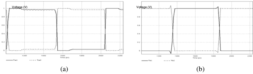
Fig. 4. The signal wave of the conventional differential mode (a) Near-end, (b) Far-end
