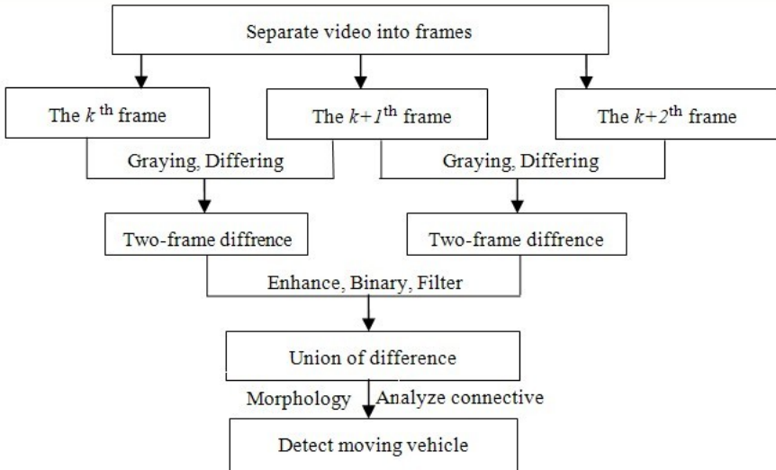
Fig. 1. Flow Chart of Three-Frame Difference
