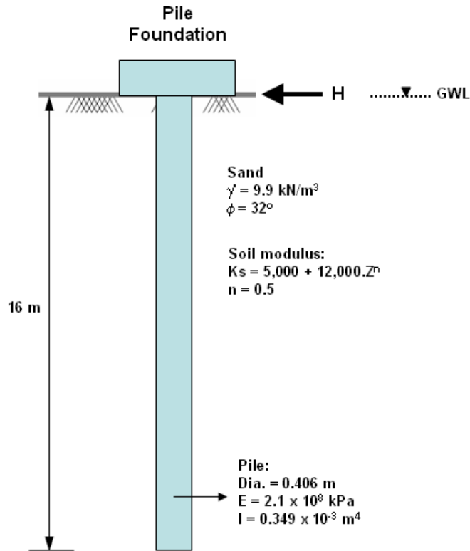
Figure 9.4: Pile foundation example
