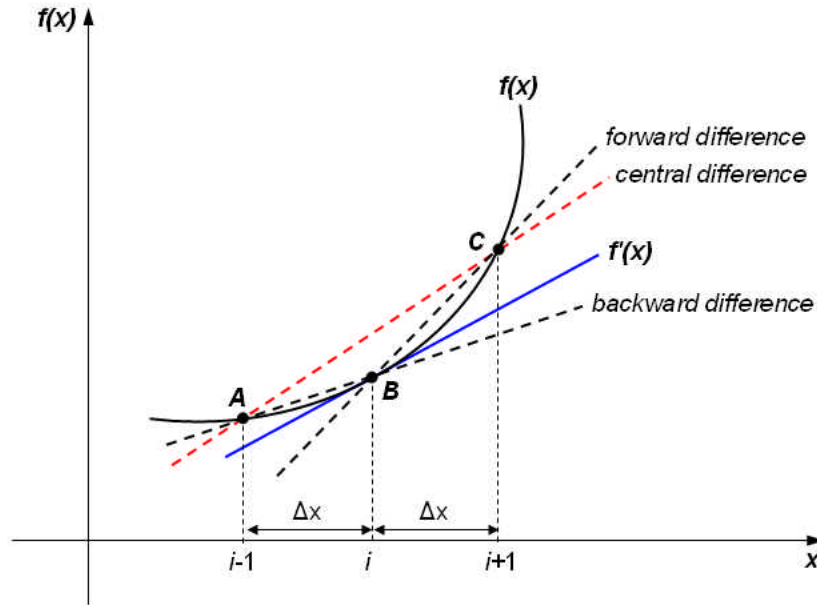
Figure 5.4: Estimation of first derivative of a function
