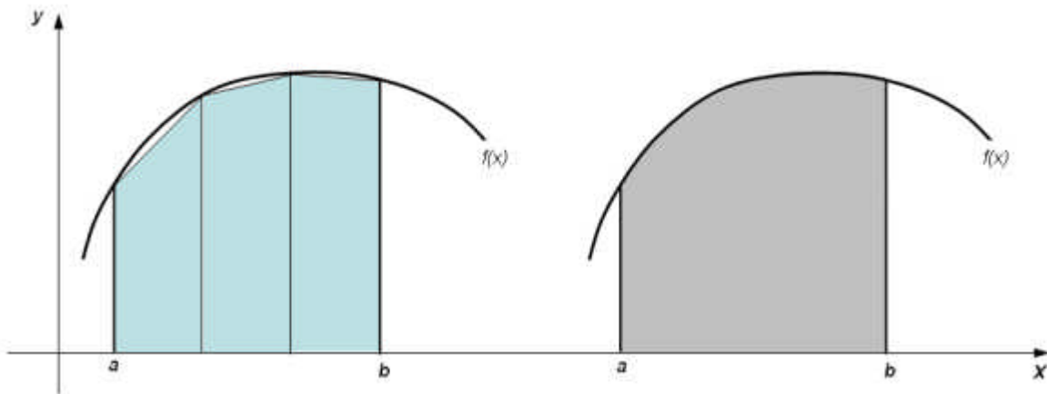
Figure 5.2: The comparison of area resulted from trapezoids (left) and the exact one (right)
