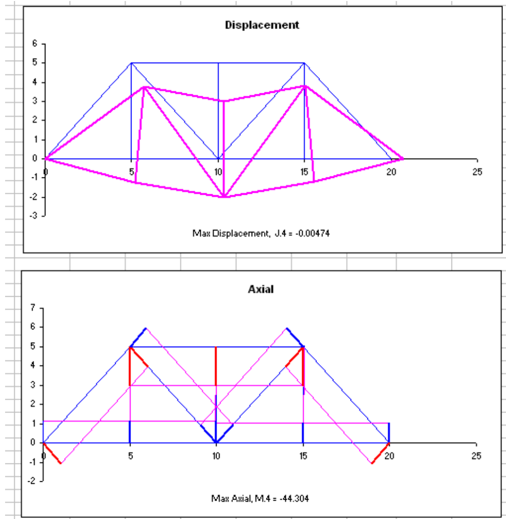
Figure 7.10: Charts of displacements and diagram of axial forces for given truss bridge
