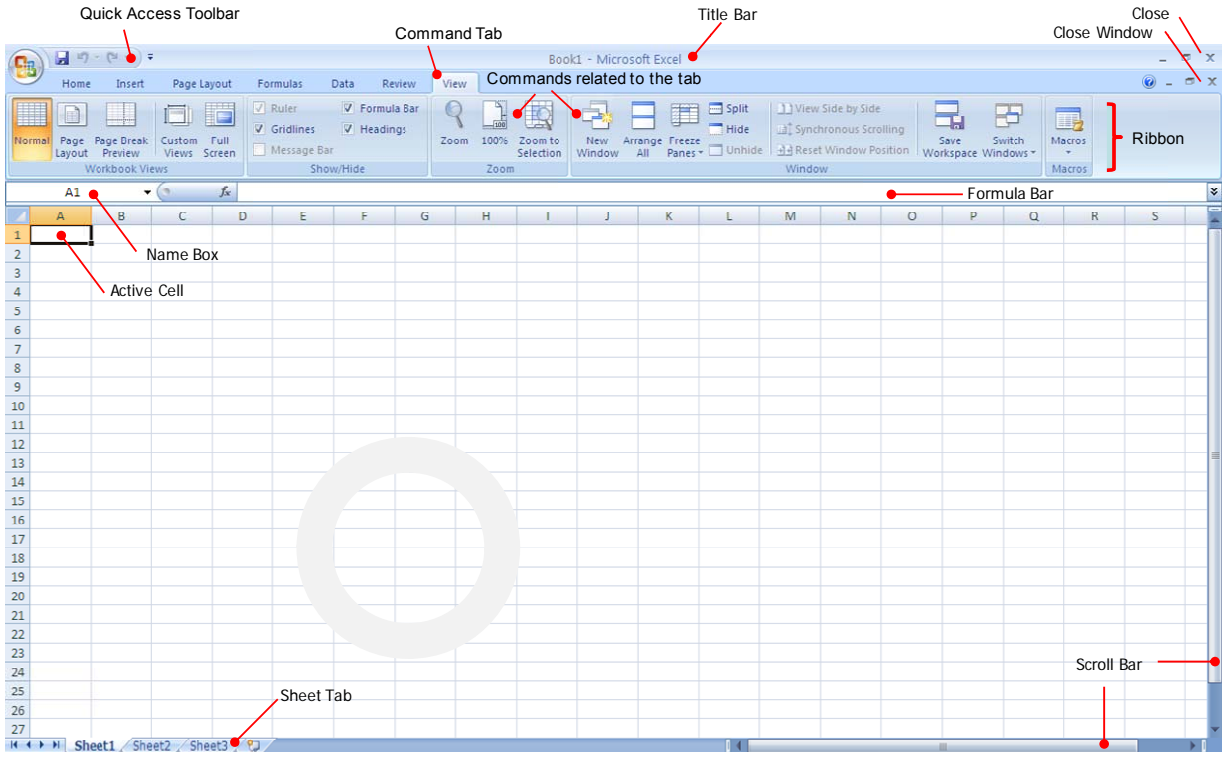
Figure 1.1: Excel 2007 Worksheet
