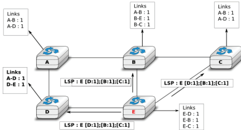
Figure 5.14: Flooding : example
