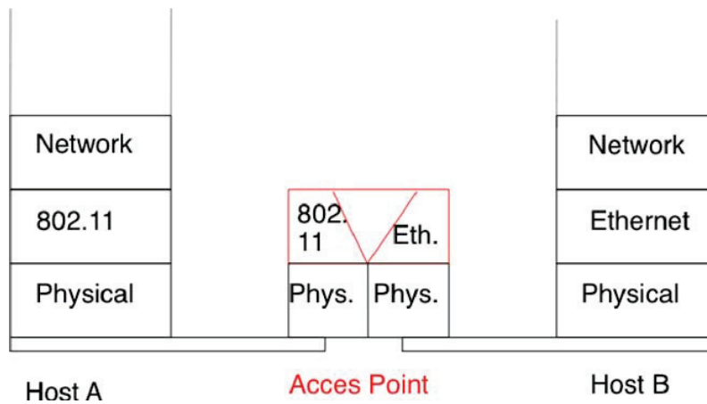
Figure 6.33: An 802.11 access point
