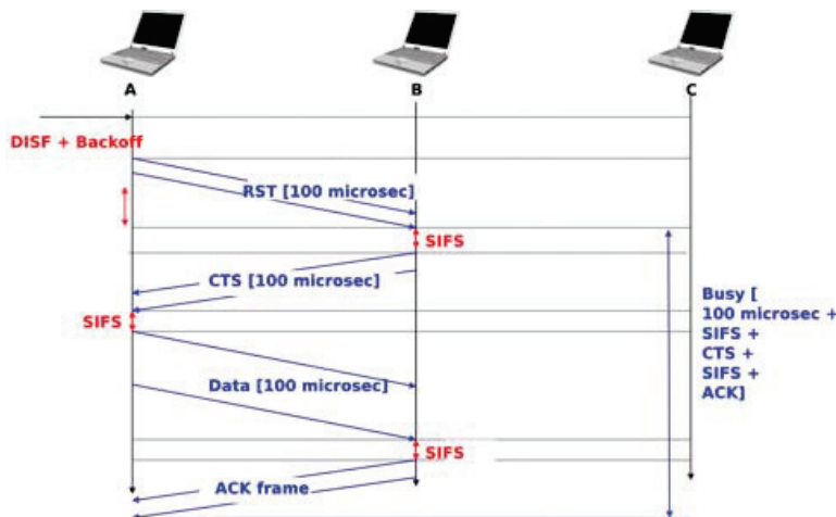
Figure 6.13: Reservations with CSMA/CA
