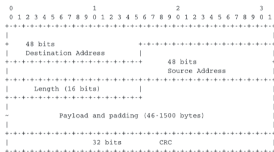
Figure 6.21: Ethernet 802.3 frame format
