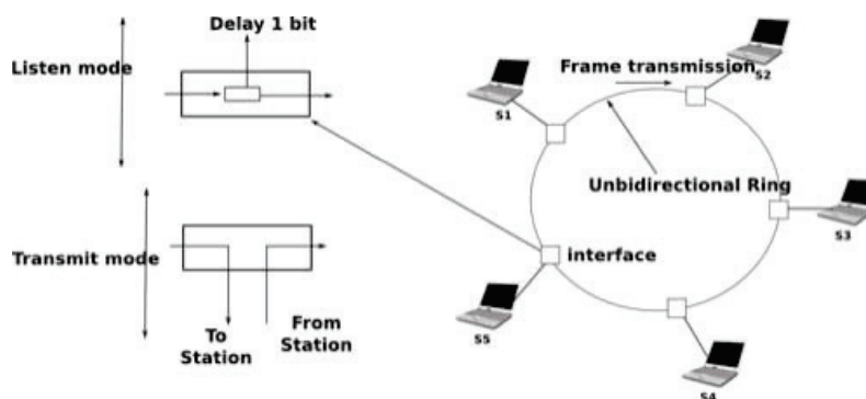
Figure 6.14: A Token Ring network
