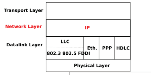
Figure 5.18: IP and the reference model
