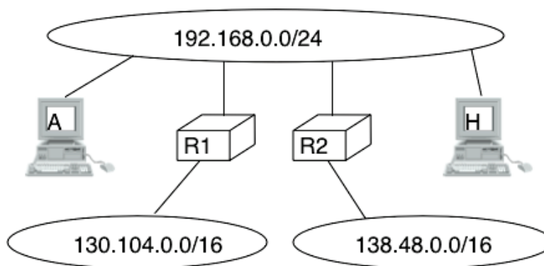
Figure 5.32: ICMP redirect
