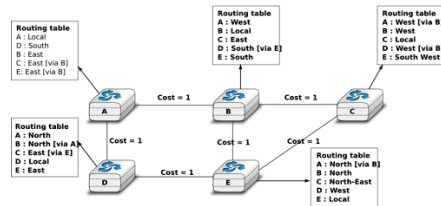
Figure 5.8: Routing tables in a simple network
