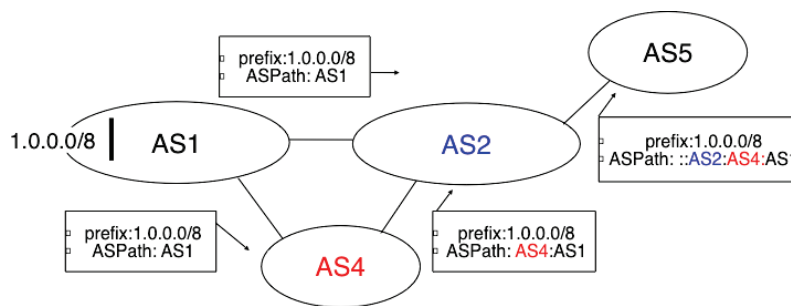
Figure 5.59: Simple exchange of BGP routes
