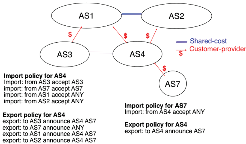
Figure 5.58: Import and export policies
