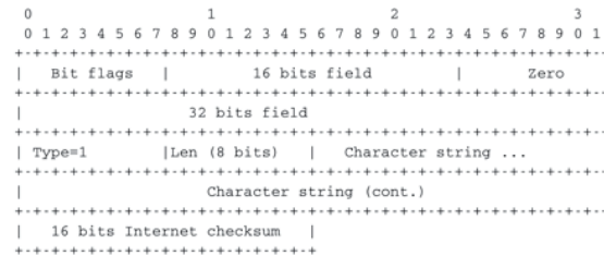
Figure 4.63: Simple SDU format
