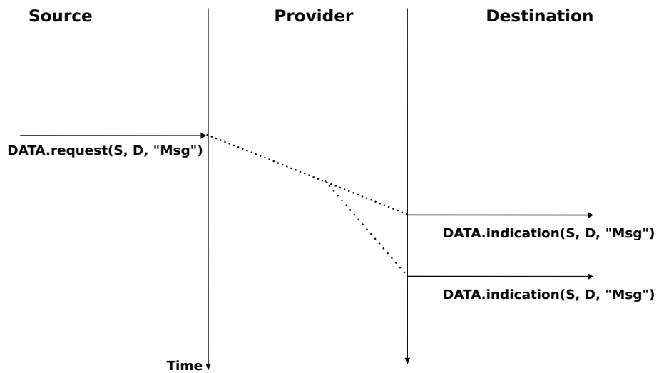
Figure 2.16: An unreliable connectionless service may duplicate SDUs
