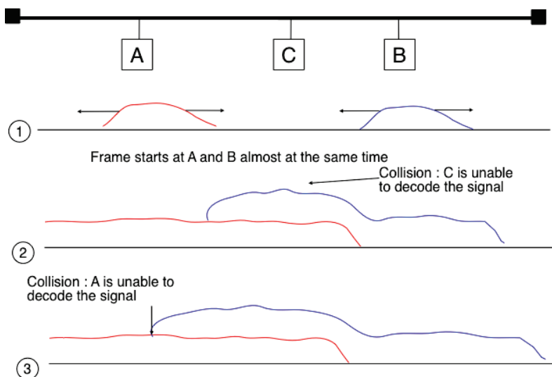
Figure 6.6: Frame collision on a shared bus
