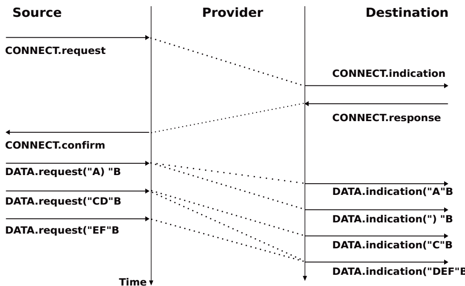
Figure 2.24: Stream-mode transfer in a connection oriented service
