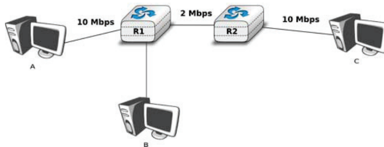
Figure 4.54: The congestion problem
