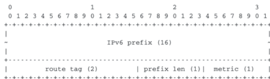
Figure 5.49: Format of the RIP IPv6 route entries
