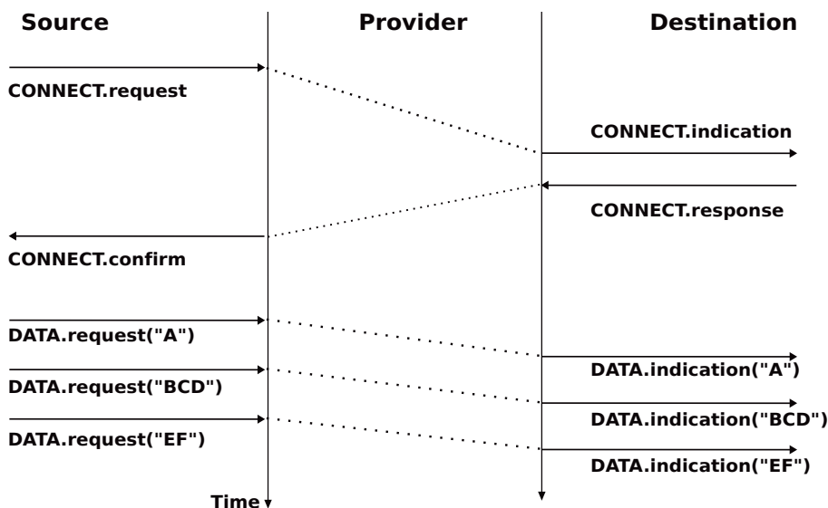
Figure 2.23: Message-mode transfer in a connection oriented service
