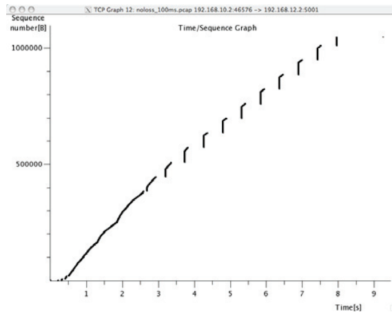
Figure 4.67: Wireshark : sequence number graph
