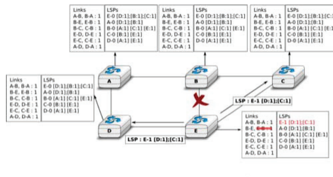
Figure 5.16: The two-way connectivity check
