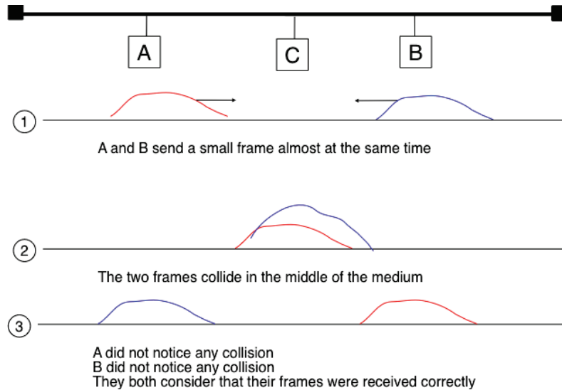
Figure 6.8: The short-frame collision problem
