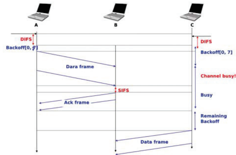
Figure 6.11: Detailed example with CSMA/CA
