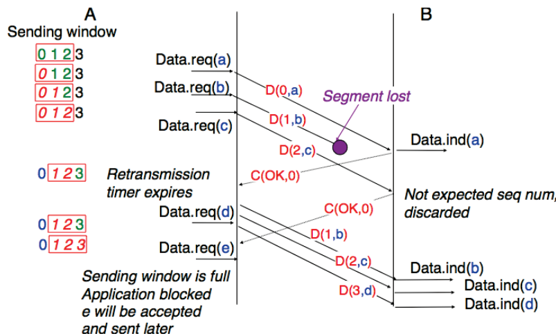
Figure 4.17: Go-back-n : example
