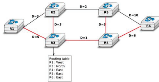
Figure 5.17: Computation of the routing table
