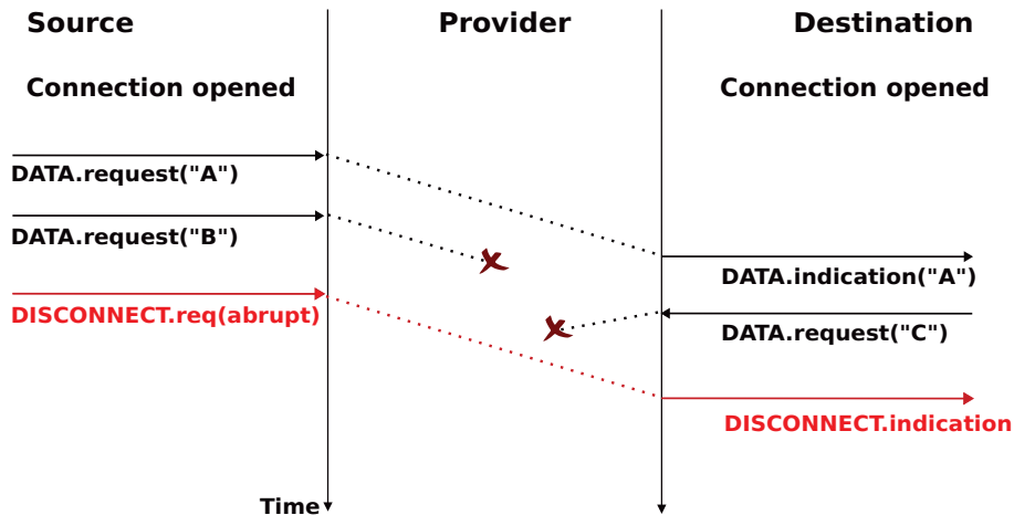
Figure 2.26: Abrupt connection release initiated by a user
