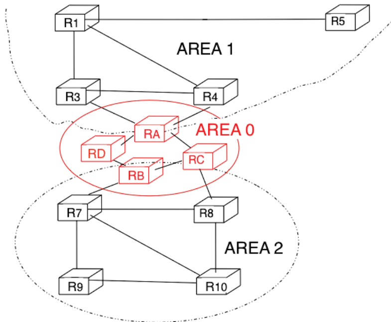
Figure 5.50: OSPF areas
