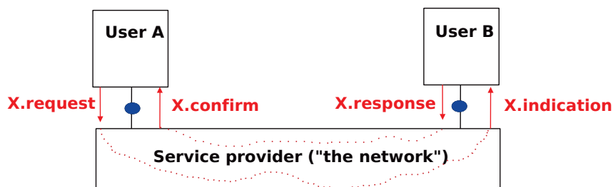
Figure 2.13: The four types of primitives
