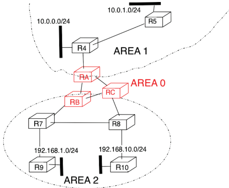
Figure 5.51: Hierarchical routing with OSPF
