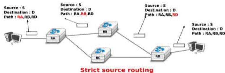
Figure 5.29: Usage of the Strict source route option
