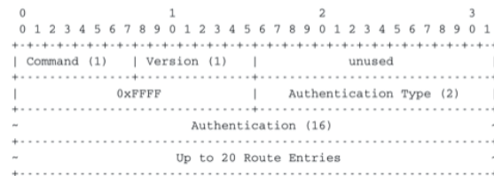
Figure 5.47: RIP message format
