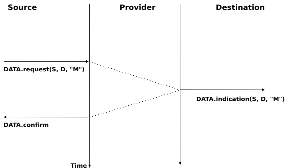
Figure 2.20: A confirmed connectionless service
