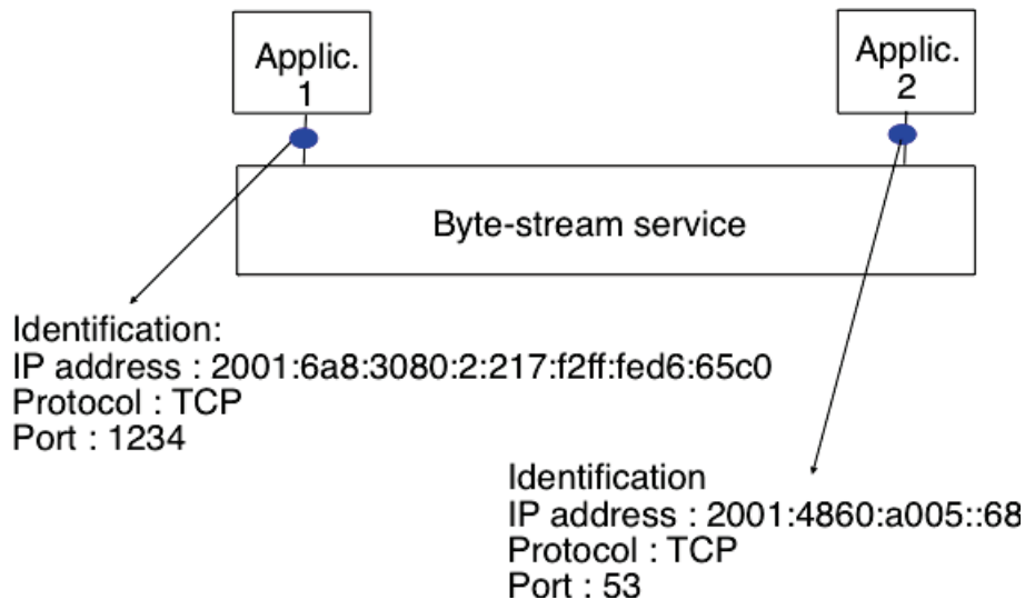
Figure 3.5: The connection-oriented or byte-stream service
