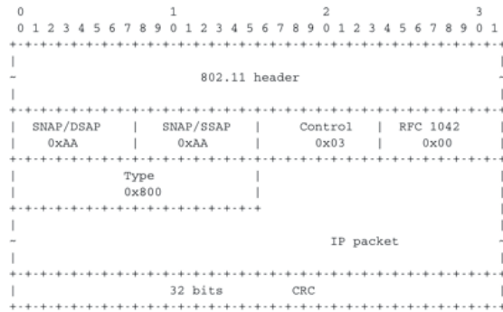
Figure 6.37: IP over IEEE 802.11
