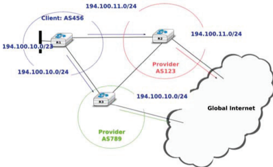
Figure 5.81: A stub connected to two providers
