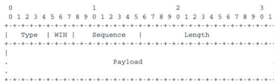
Figure 4.64: Segment format
