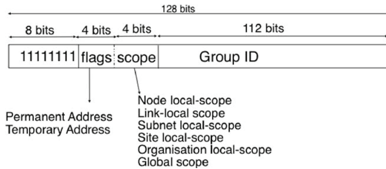
Figure 5.38: IPv6 multicast address structure
