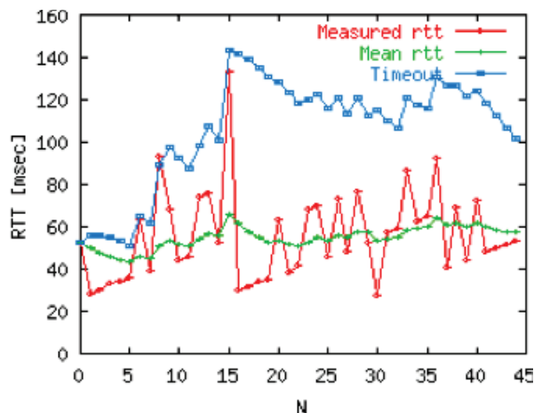
Figure 4.47: Example computation of the rto
