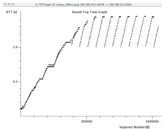
Figure 4.68: Wireshark : round-trip-time graph
