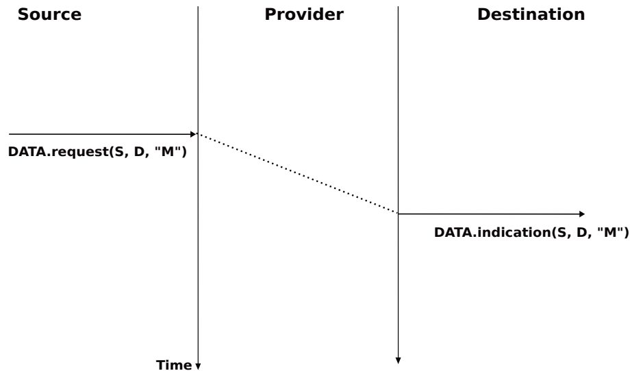
Figure 2.14: A simple connectionless service
