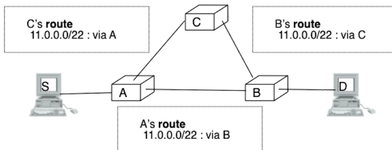
Figure 5.27: Forwarding loops in an IP network
