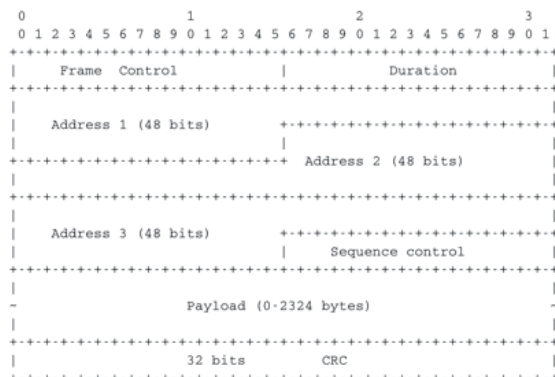
Figure 6.34: 802.11 data frame format
