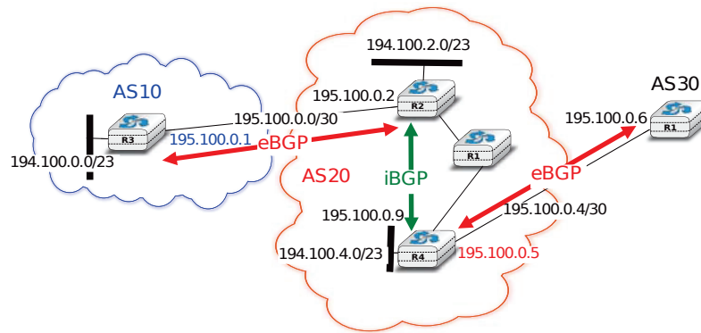
Figure 5.65: How to deal with non-BGP routers ?
