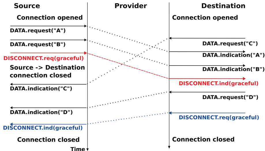
Figure 2.27: Graceful connection release
