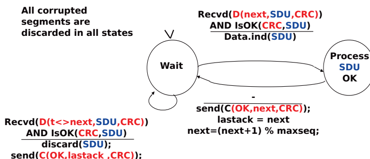
Figure 4.15: Go-back-n : receiver FSM
