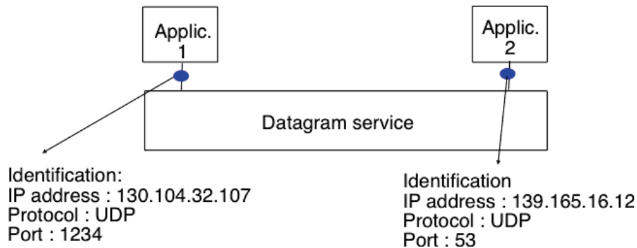
Figure 3.4: The connectionless or datagram service
