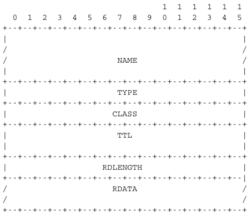
Figure 3.10: DNS Resource Records
