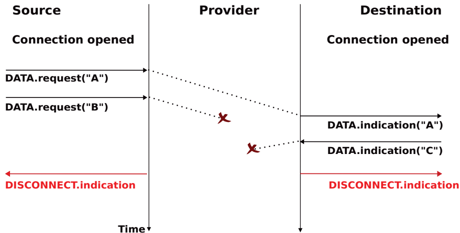
Figure 2.25: Abrupt connection release initiated by the service provider
