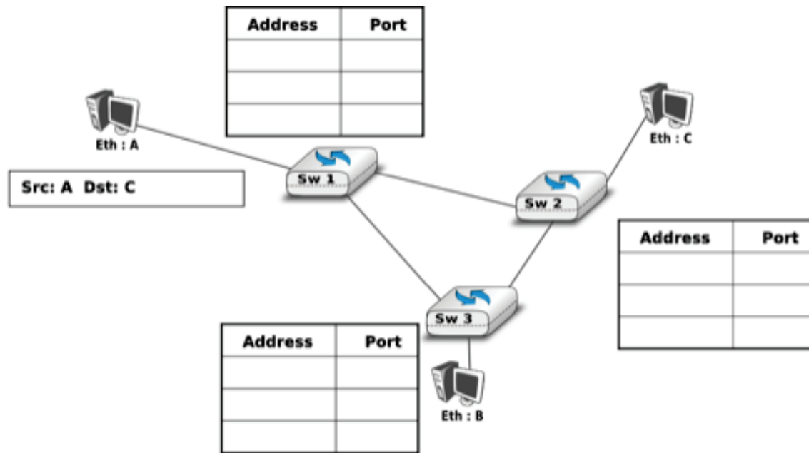
Figure 6.26: Ethernet switches in a loop
