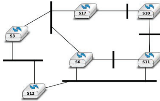
Figure 6.38: A small network composed of Ethernet switches
