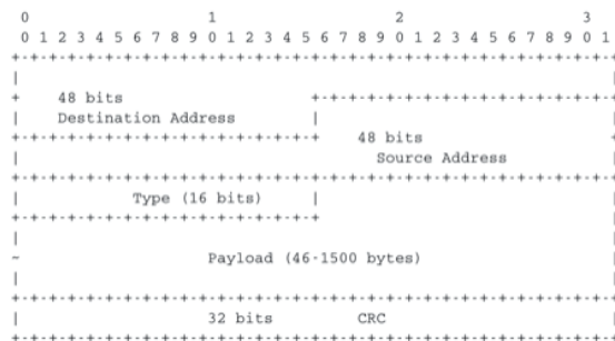
Figure 6.20: Ethernet DIX frame format
