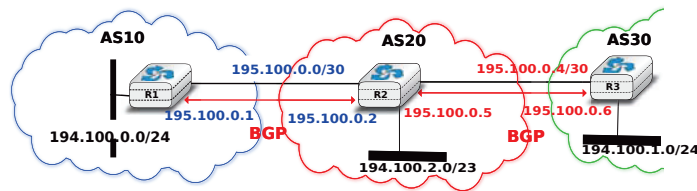
Figure 5.62: Utilisation of the BGP nexthop attribute
