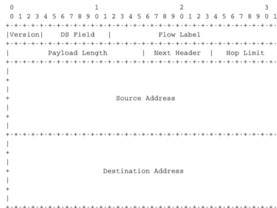
Figure 5.39: The IP version 6 header ( RFC 2460 )
