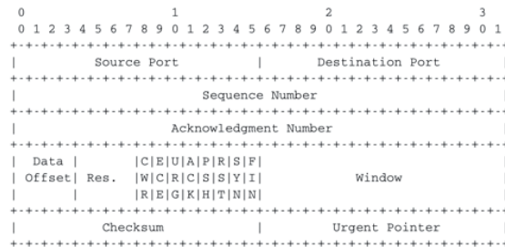
Figure 4.36: TCP header format
