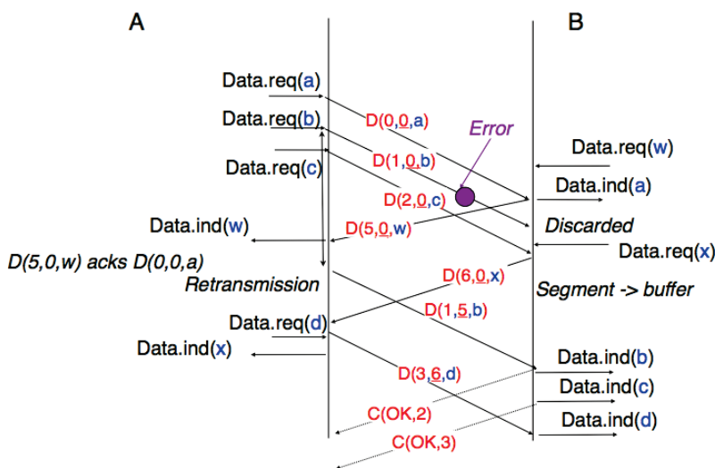
Figure 4.23: Piggybacking
