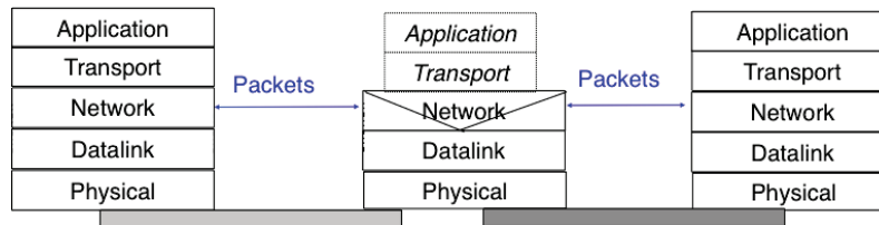
Figure 5.43: IP middleboxes and the reference model
