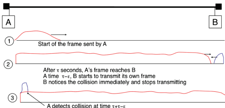
Figure 6.7: The worst collision on a shared bus
