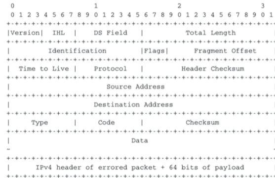
Figure 5.31: ICMP version 4 ( RFC 792 )
