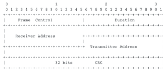
Figure 6.36: IEEE 802.11 RTS frame format
