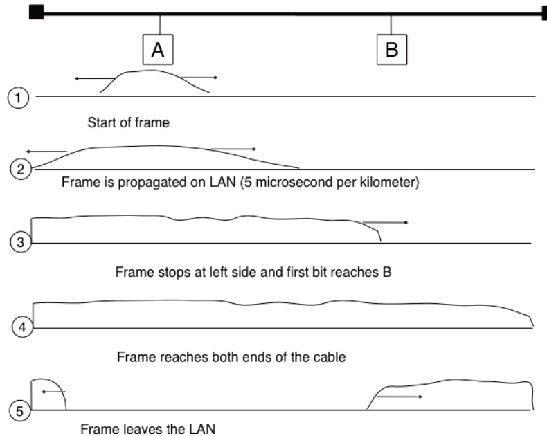
Figure 6.5: Frame transmission on a shared bus
