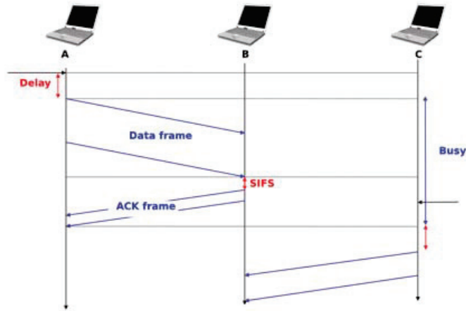
Figure 6.9: Operation of a CSMA/CA device
