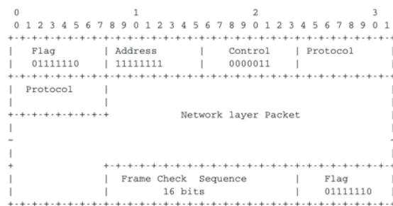
Figure 6.17: PPP frame format
