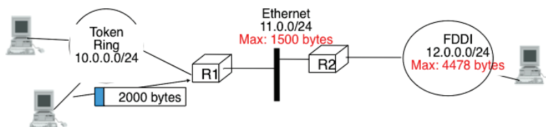
Figure 5.28: The need for fragmentation and reassembly
