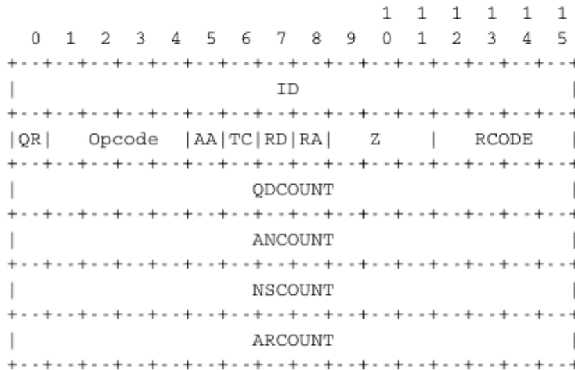
Figure 3.9: DNS header
