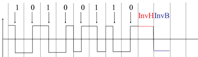
Figure 6.2: Manchester encoding
