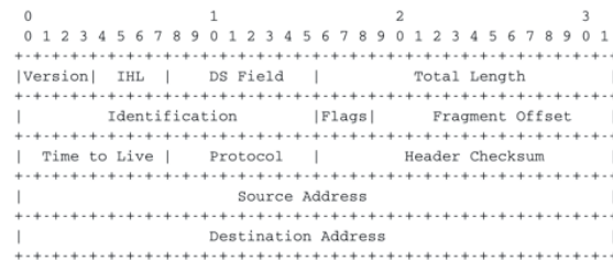
Figure 5.26: The IP version 4 header
