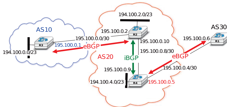
Figure 5.64: iBGP and eBGP sessions
