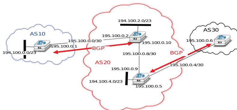
Figure 5.63: A larger network using BGP
