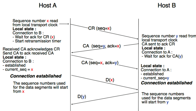
Figure 4.28: Three-way handshake
