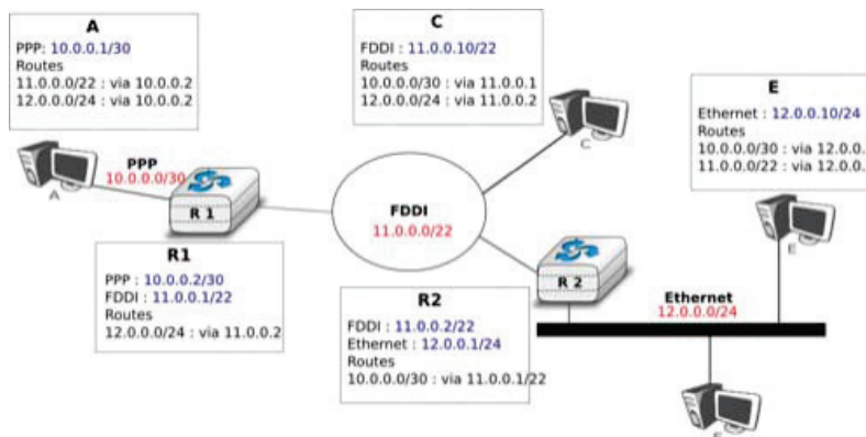
Figure 5.21: IP subnets in a simple enterprise network
