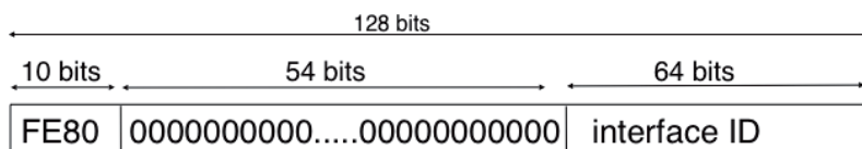
Figure 5.37: IPv6 link local address structure
