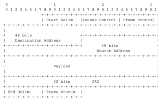
Figure 6.16: 802.5 data frame format
