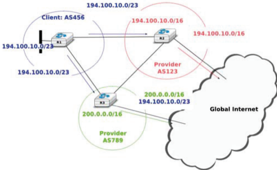
Figure 5.80: A stub connected to two providers
