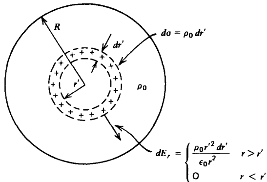
Figure 2-17 (a) Gaussian spheres for a uniformly charged sphere show that the electric field outside the sphere is again the same as if all the charge Q = \frac{4}{3}\pi R^3 \rho_0 were concentrated as a point charge at r = 0 . (b) The solution is also obtained by summing the contributions from incremental spherical shells of surface charge.
