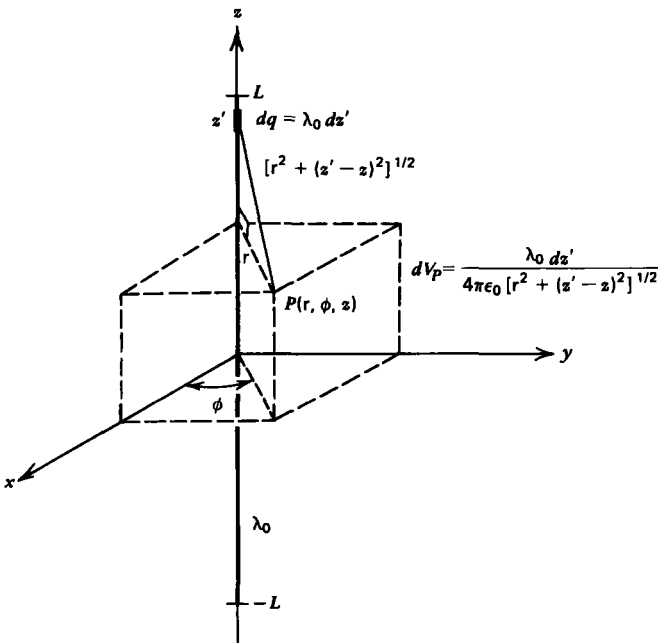
Figure 2-21 The potential from a finite length of line charge is obtained by adding the potentials due to each incremental line charge element.
