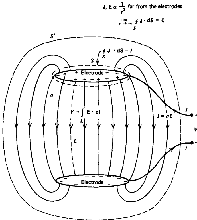
Figure 3-15 A voltage applied across two electrodes within an ohmic medium causes a current to flow into one electrode and out the other. The electrodes have equal magnitude but opposite polarity charges so that far away the fields die off as a dipole \propto (1/r^3) . Then, even though the surface S' is increasing as r^2 , the flux of current goes to zero as 1/r .
