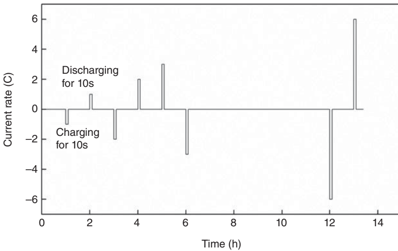
Figure 4.3 The current curve for the JEVS test.
