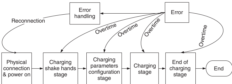
Figure 7.33 Charge flow.
