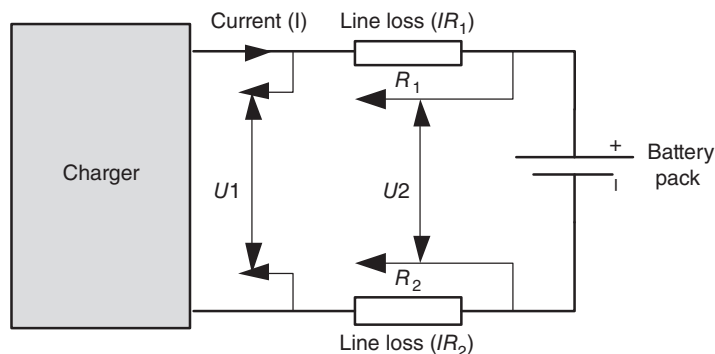
Figure 5.1 Schematic diagram of the charger-alone control mode.
