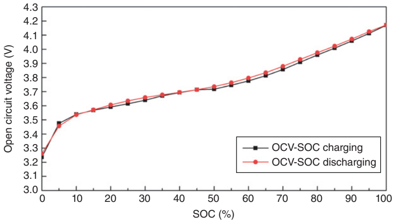
Figure 4.16 Plot of OCV versus SOC for a power lithium manganese battery. Reproduced with permission from Hongyu Guo, “Research on Power Capability Prediction Method of HEV Lithium-ion Battery,” Beijing Jiaotong University © 2012
