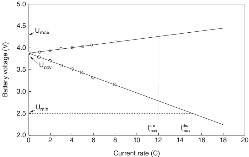
Figure 4.4 Voltage versus current for the JEVS test.
