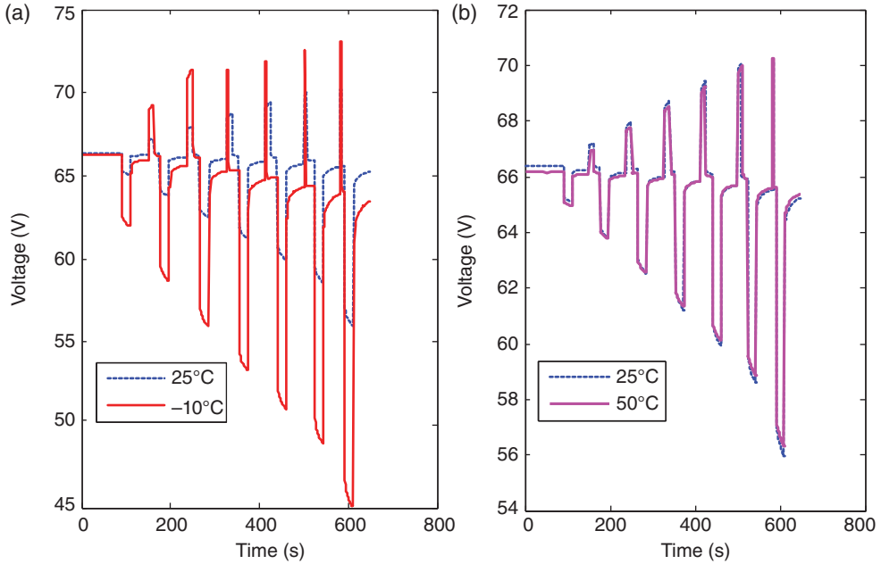
Figure 2.22 Comparison of voltage responses under composite pulse working condition between (a) low temperature ( -10\text{ }^{\circ}\text{C} ) and room temperature ( 25\text{ }^{\circ}\text{C} ) and (b) high temperature ( 50\text{ }^{\circ}\text{C} ) and room temperature. (Reproduced with permission from Caiping Zhang, “State of Charge Estimation and Peak Power Capability Predict of Lithium-Ion Batteries for Electric Transmission Vehicles”, Beijing Institute of Technology, ©2010.)
