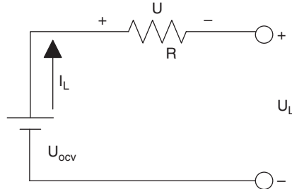
Figure 2.13 Circuit structure of Rint model.
