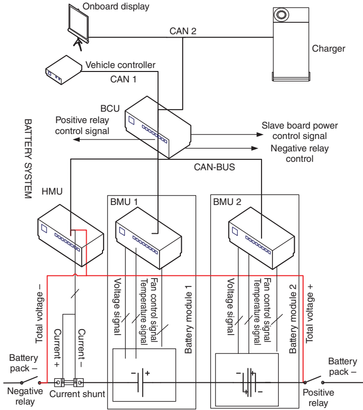
Figure 7.41 The BMS structure of the Tongyue BEV.
