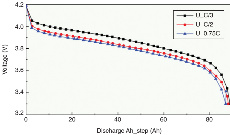
Figure 3.1 Discharge curves with different discharge currents.
