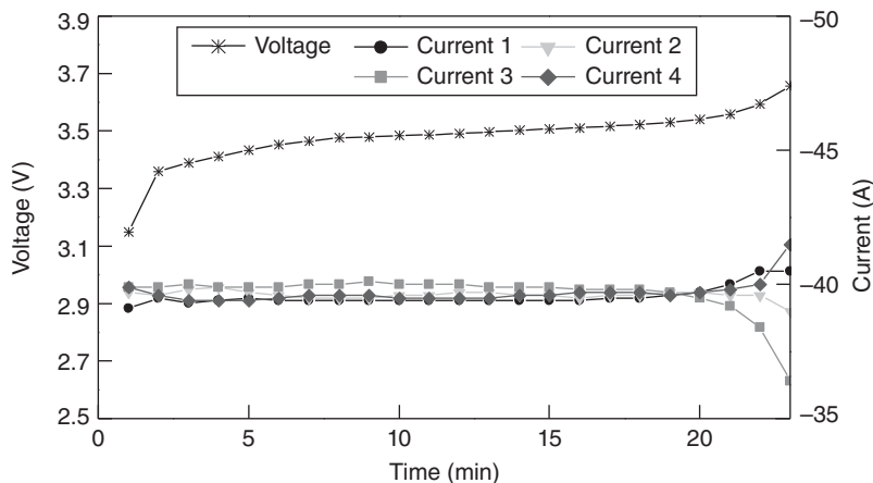
Figure 6.6 The unbalanced current of a \text{LiFePO}_4 parallel-connected battery with a charge rate of 1.5 C.
