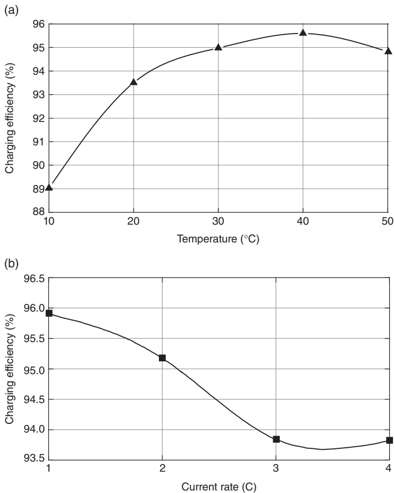
Figure 5.5 Charging efficiency (Wh) (a) at different temperatures and (b) with different charging rates.
