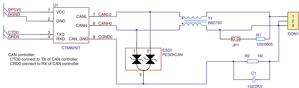
Figure 7.29 The interface hardware circuit of the CAN bus based on CTM.
