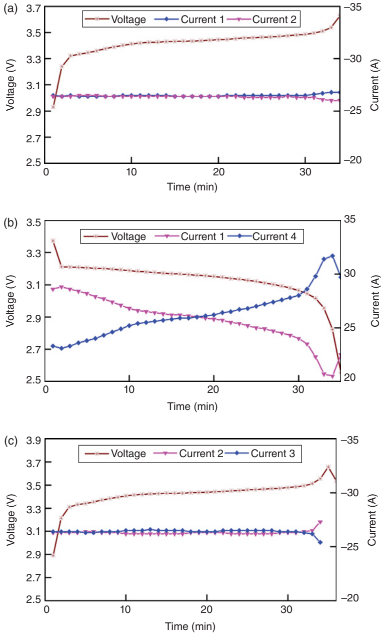
Figure 6.7 The unbalanced charging current of a \text{LiFePO}_4 parallel-connected battery with a charge rate of 1 C. Batteries connected in parallel: (a) 1 and 2, (b) 1 and 4, (c) 2 and 3.
