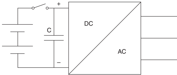
Figure 7.18 Battery pack connection with inverter.
