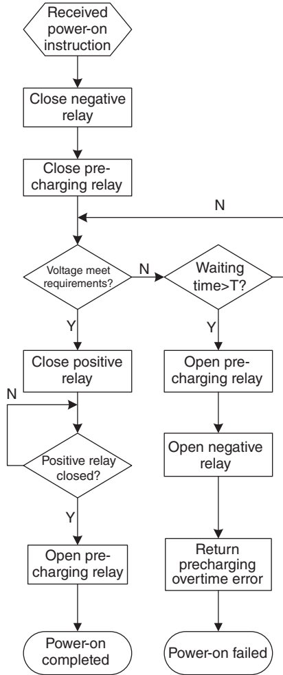
Figure 7.32 The high voltage power-up flow.
