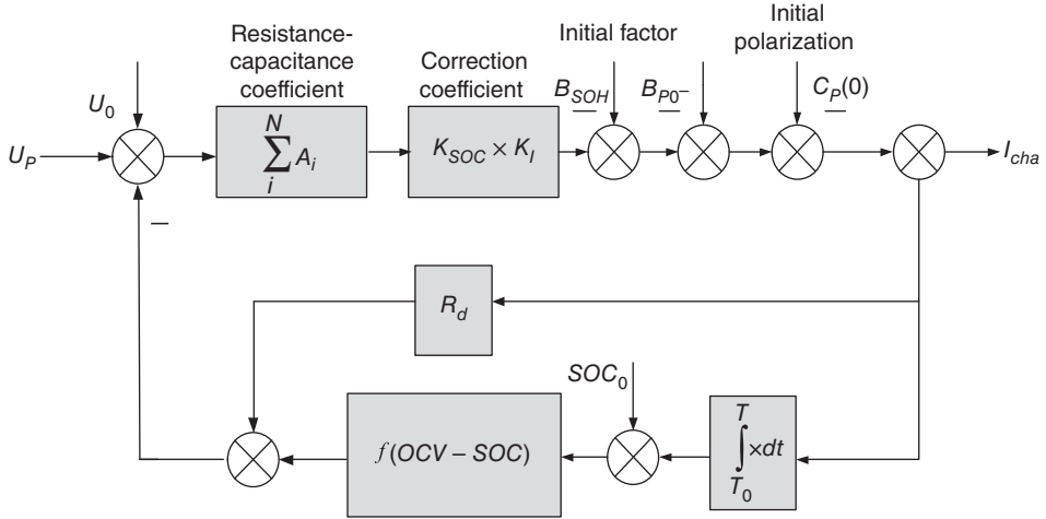
Figure 5.27 The polarization voltage control logic diagram.
