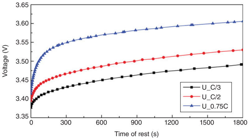
Figure 3.2 Restoring curves of voltage with different currents.
