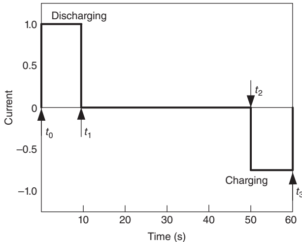
Figure 2.18 HPPC cycling process.
