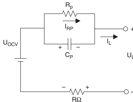
Figure 2.14 Circuit structure of Thevenin model.
