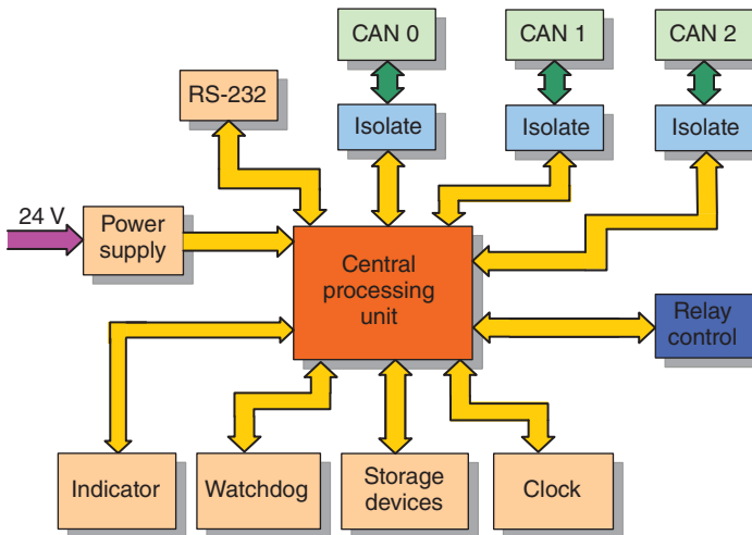
Figure 7.4 The hardware circuit structure of the BCU.
