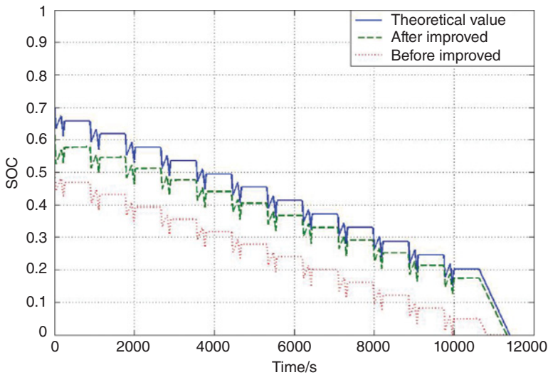
Figure 3.30 Simulation comparison before and after the improvement of the EKF algorithm under the working condition of the self-defined compound pulse.
