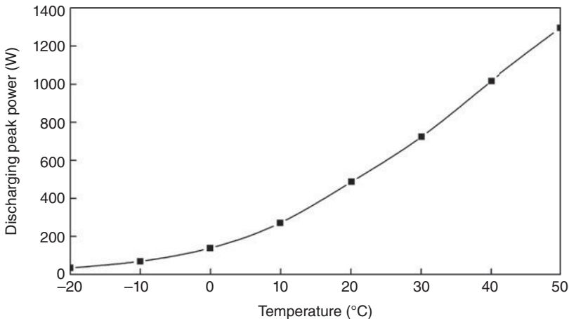
Figure 4.11 Plot of discharging peak power versus temperature with 60% SOC.
