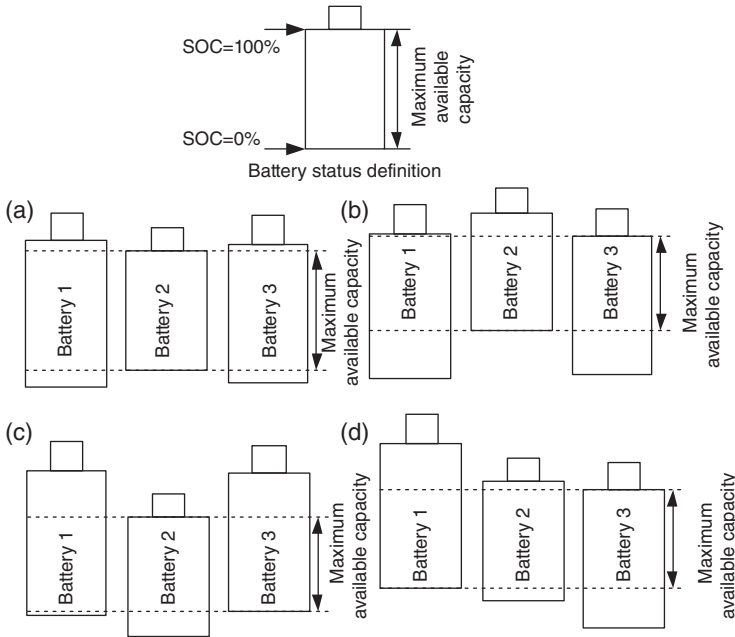
Figure 6.21 Judgment criteria for equalization of the battery.
