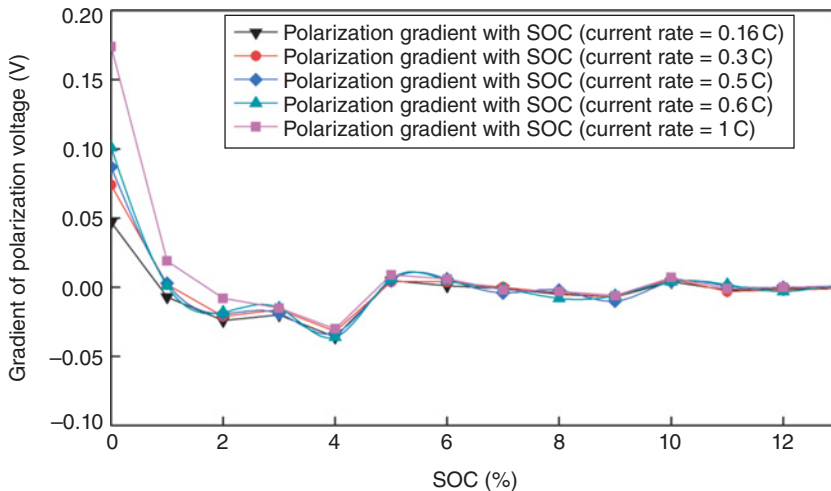
Figure 5.14 SOC gradients of the polarization voltage at different initial currents. Reproduced with permission from Jiapeng Wen, “Studies of Lithium-ion Power Battery optimization charging theory for Pure Electric Vehicle,” Beijing Jiaotong University, @2011
