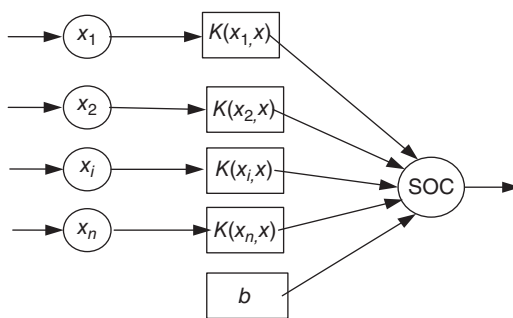
Figure 3.13 Model structure of support vector regression.
