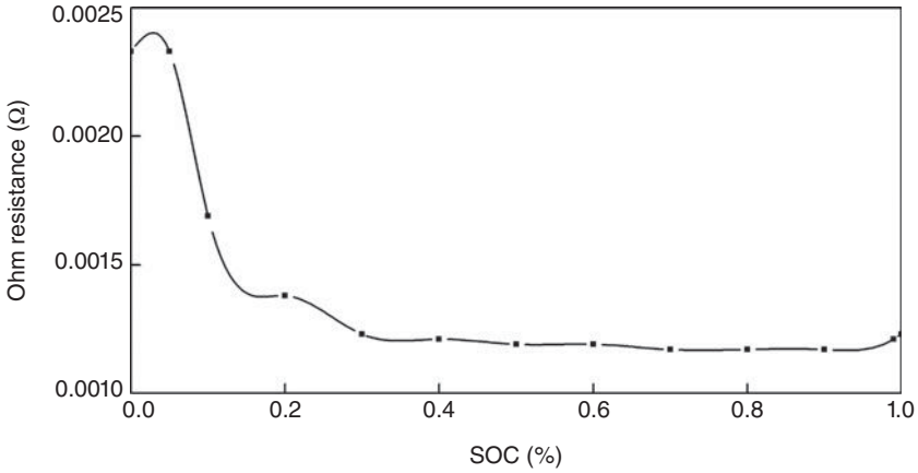
Figure 2.3 Ohmic resistance changes with SOC.
