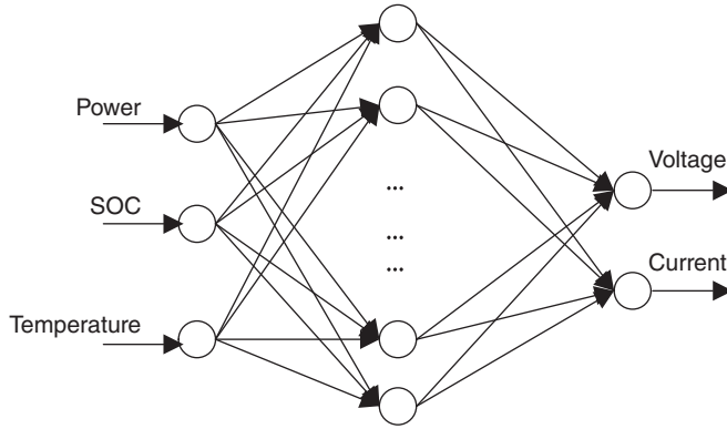
Figure 2.17 Structure of neural network model with power to be input.
