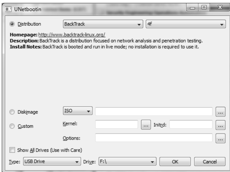
Figure 7-3 UNetbootin interface
