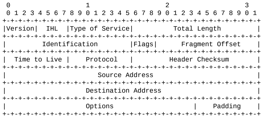
Example Internet Datagram Header
