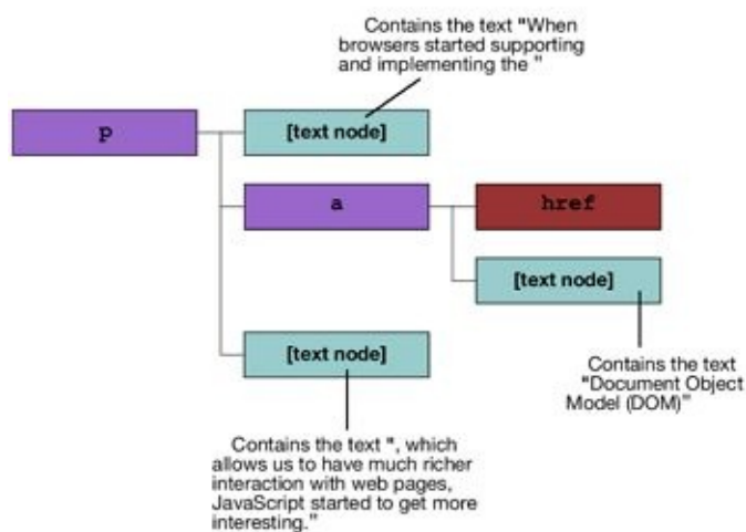
Figure 2: A visual representation of our sample DOM tree.
