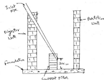
Fig 4.3 Inlet and outlet Pipes
