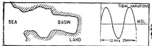
Fig 5.1 Single basin Tidal Power Plant
