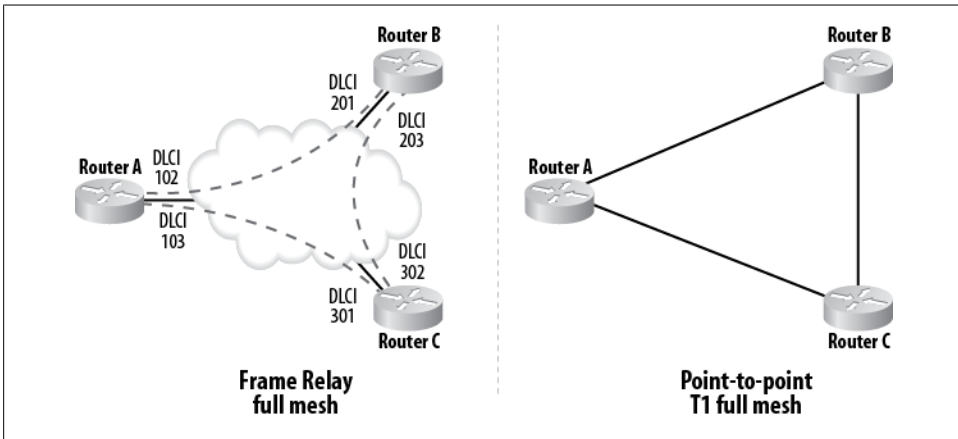
Figure 23-6. Frame Relay versus point-to-point T1 meshed networks
