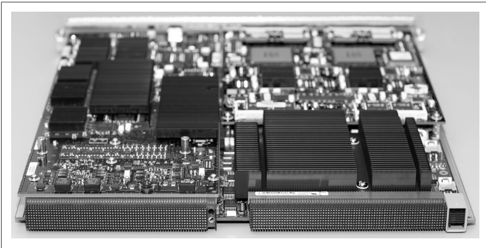
Figure 17-5. Supervisor-720 connectors
