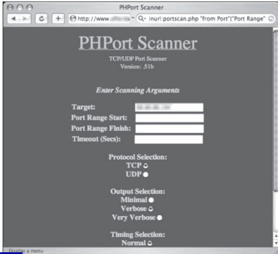
Figure 6.3 PHPPort Scanner-A Nifty Web-Based Portscanner
