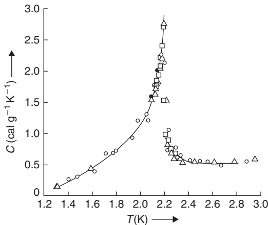
FIGURE 7.5 The specific heat of liquid \text{He}^4 under its own vapor pressure (after Keesom and coworkers).
